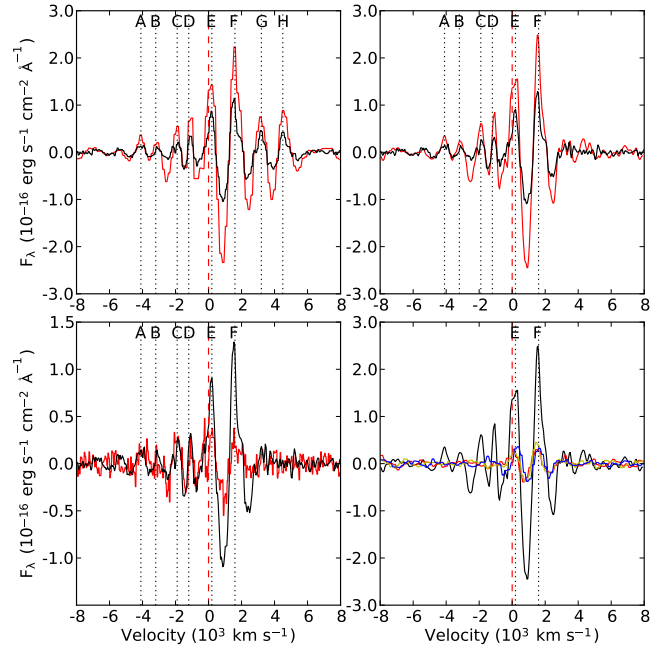
Fig. 14. Comparison of large scale subtracted line profiles. The upper left panel shows the [O I] 6300, 6364 Å line at days 202 (red) and 300 (black). The upper right panel shows the decomposed [O I] 6300 Å line at days 202 (red) and 300 (black). The lower left panel shows the decomposed [O I] 6300 Å line (black) and the Mg I 4571 Å line (red) at day 300. The lower right panel shows the decomposed [O I] 6300 Å line (black) and the [O I] 5577 Å (red), O I 7774 Å (green), and Na I 5890, 5896 Å (blue) lines at day 202.
