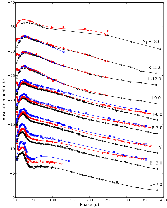
Fig. 2. Absolute optical, NIR, and MIR broad-band lightcurves before day 400 for SNe 2011dh (black circles), 1993J (red triangles), and 2008ax (blue squares). For clarity each band has been shifted in magnitude and the lightcurve annotated with the shift applied. We also show combinations of spline fits, interpolations, and extrapolations (solid lines) used e.g. in the calculations of the pseudo-bolometric lightcurves.
