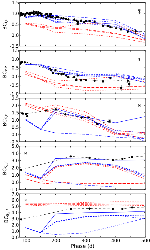
Fig. 20. Observed (black circles) and J14 model pseudo-BCs between days 100 and 500 for the I , z , K , S_1 , and S_2 bands. The model families differing in molecular cooling (complete, red; none, blue) and the optical depth of the dust (0, long-dashed; 0.25, short-dashed; 0.44, solid) are shown. 17 M_{\odot} and medium mixing models are not shown. The error bars arising from the extinction are marked in the upper left or right corner.
