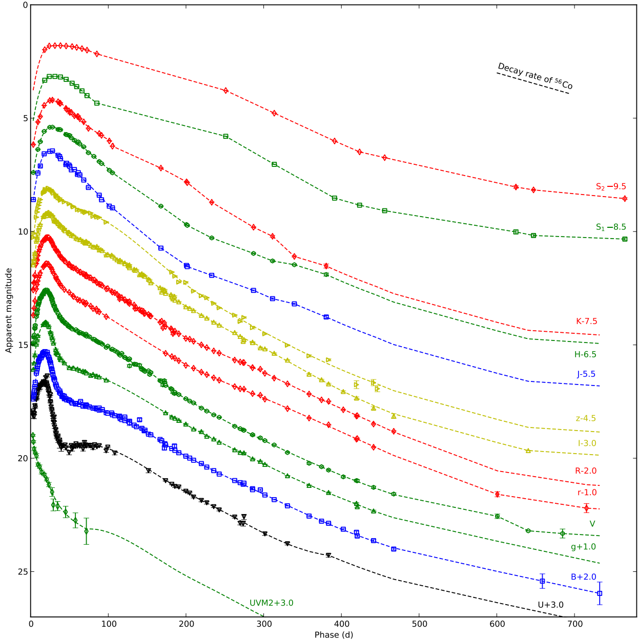
Fig. 1. Apparent UV, optical, NIR, and MIR broad-band lightcurves before day 800 for SN 2011dh. For clarity each band has been shifted in magnitude and the lightcurve annotated with the shift applied. We also show combinations of spline fits, interpolations, and extrapolations (dashed lines) used e.g. in the calculations of the pseudo-bolometric lightcurves.
