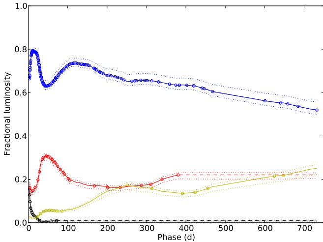
Fig. 5. Fractional UV (black dots), optical (blue dots), NIR (red dots), and MIR (yellow dots) luminosity before day 750 for SN 2011dh. Interpolations and extrapolations are shown as solid and dashed lines, respectively. The upper and lower error bars for the systematic error arising from extinction (dotted lines) are also shown.
