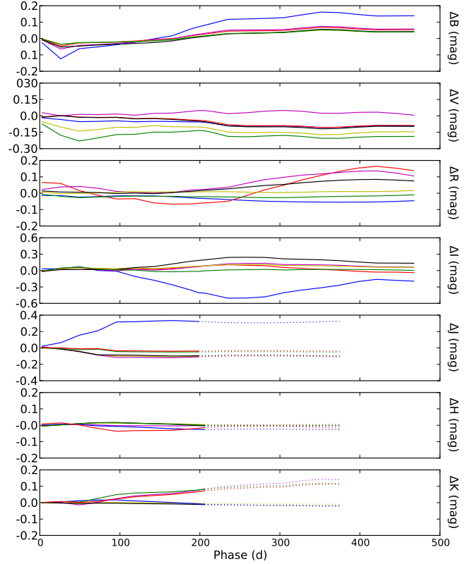
Fig. A.1. Difference between JC BVRI colour and S-corrections for NOT/ALFOSC (black), LT/RATCam (red), CA-2.2 m/CAFOS (blue), TNG/LRS (green), AS-1.82 m/AFOSC (yellow), and AS-Schmidt (magenta), and difference between 2MASS JHK colour and S-corrections for NOT/NOTCAM (black), TCS/CAIN (red), CA-3.5 m/O2000 (blue), TNG/NICS (green), WHT/LIRIS (yellow), and UKIRT/WFCAM (magenta). Results based on extrapolated 2MASS S-corrections are shown as dotted lines.
