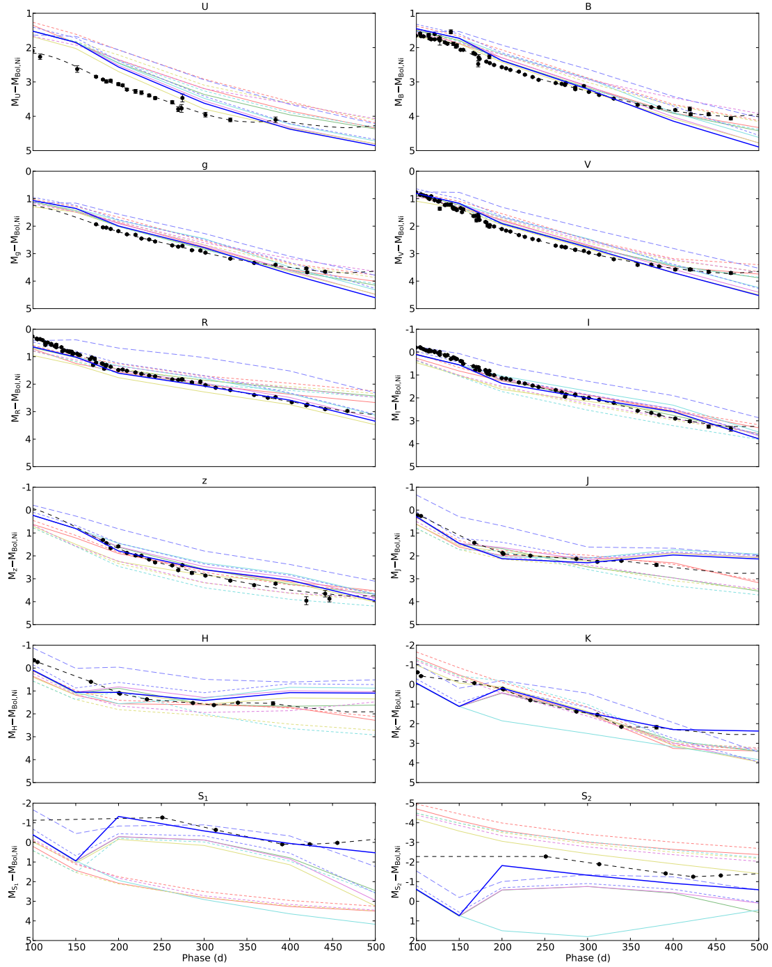
Fig. 17. Observed (black circles) and J14 model optical, NIR, and MIR (absolute) magnitudes between days 100 and 500 normalized to the radioactive decay chain luminosity of 0.075 M_{\odot} of ^{56}\text{Ni} . The preferred model (12F) is shown as a blue solid line. The other models are shown in shaded colour as follows: 12A (red solid line), 12B (green solid line), 12C (magenta solid line), 12D (yellow solid line), 12E (cyan solid line), 13A (red short-dashed line), 13C (yellow short-dashed line), 13D (cyan short-dashed line), 13E (magenta short-dashed line), 13G (blue short-dashed line), 17A (blue long-dashed line).
