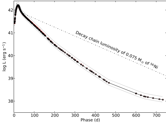
Fig. 4. UV-to-MIR pseudo-bolometric lightcurve before day 750 for SN 2011dh (black circles and solid line). The upper and lower error bars for the systematic error arising from extinction and distance (black dotted lines) and the radioactive decay chain luminosity of 0.075 M_{\odot} of ^{56}\text{Ni} (black dash-dotted line) are also shown.
