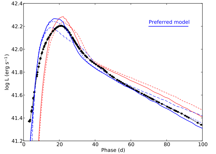
Fig. 18. J14 model bolometric lightcurves between days 3 and 100 calculated with HYDE, compared to the observed optical-to-MIR pseudo-bolometric lightcurve (black circles). The model families differing in initial mass ( 12 M_{\odot} , solid; 13 M_{\odot} , short-dashed; 17 M_{\odot} , long-dashed) and macroscopic mixing (medium, red; strong, blue) are shown. Following this coding, the preferred model is shown as a blue solid line.
