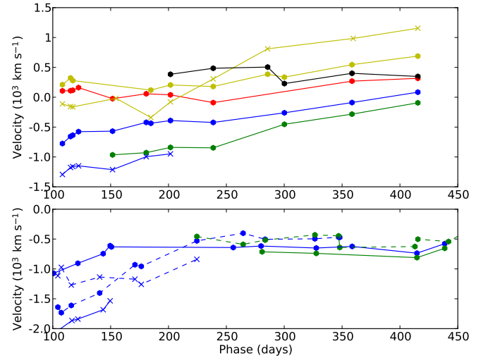
Fig. 13. Upper panel: center of flux velocities for the [O I] 6300, 6364 Å (blue circles), [O I] 5577 Å (blue crosses), Mg I 4571 Å (green circles), [Ca II] 7291, 7323 Å (yellow circles), Ca II 8498, 8542, 8662 Å (yellow crosses), Na I 5890, 5896 Å (red circles), and [Fe II] 7155 Å (black circles) lines for SN 2011dh. Lower panel: center of flux velocities for the [O I] 6300, 6364 Å (blue circles), [O I] 5577 Å (blue crosses), and Mg I 4571 Å (green circles) lines for SNe 1993J (dashed lines) and 2008ax (solid lines).
