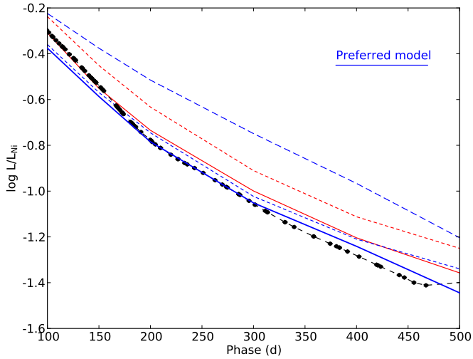
Fig. 15. Observed (black circles) and J14 model optical-to-MIR pseudo-bolometric lightcurves between days 100 and 500 normalized to the radioactive decay chain luminosity of 0.075 M_{\odot} of ^{56}\text{Ni} . Selected representatives (12A, 12F, 13A, 13C, 17A) of the model families differing in initial mass ( 12 M_{\odot} , solid; 13 M_{\odot} , short-dashed; 17 M_{\odot} , long-dashed) and macroscopic mixing (medium, red; strong, blue) are shown. Following this coding, the preferred model is shown as a blue solid line.
