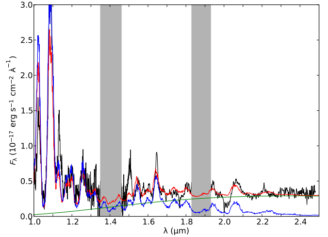
Fig. 21. Observed zJ and HK spectra at days 198 and 206 (black) compared to NIR spectra for the preferred model (12F, red) and model 12E (blue), which differs only in that \tau_{\text{dust}} = 0 . The observed spectra were flux calibrated with the interpolated observed J , H , and K magnitudes at day 200 and we also show the dust emission component for the preferred model (green).
