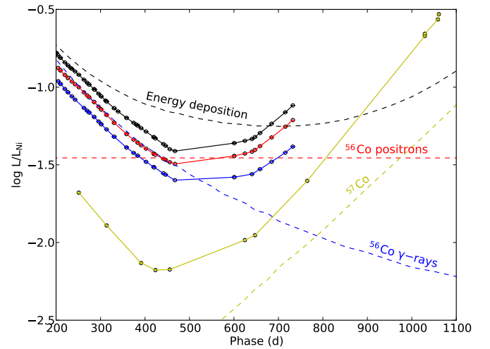
Fig. 23. Optical-to-MIR (black dots), optical-plus-MIR (red dots), optical (blue dots), and MIR (yellow dots) pseudo-bolometric lightcurves after day 200, compared to the bolometric lightcurve (black dashed line), deposited ^{56}\text{Co} \gamma -ray (blue dashed line) and positron (red dashed line) luminosity, and deposited ^{57}\text{Co} luminosity (yellow dashed line) for the preferred steady-state NLTE model (12F). The lightcurves have been normalized to the radioactive decay chain luminosity of 0.075 M_{\odot} of ^{56}\text{Ni} .
