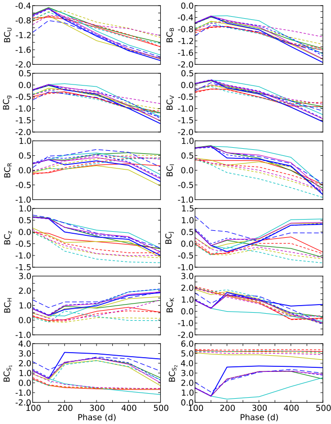
Fig. C.2. Broad-band BCs between days 100 and 500 for the J14 models. The models are shown as in Fig. 17.
