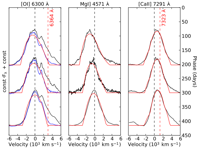
Fig. 11. [O I] 6300, 6364 Å (left panel; black), decomposed [O I] 6300 Å (left panel; blue), Mg I 4571 Å (middle panel; black), and [Ca II] 7291, 7323 Å (right panel; black) lines at selected epochs, compared to line profile fits (red).
