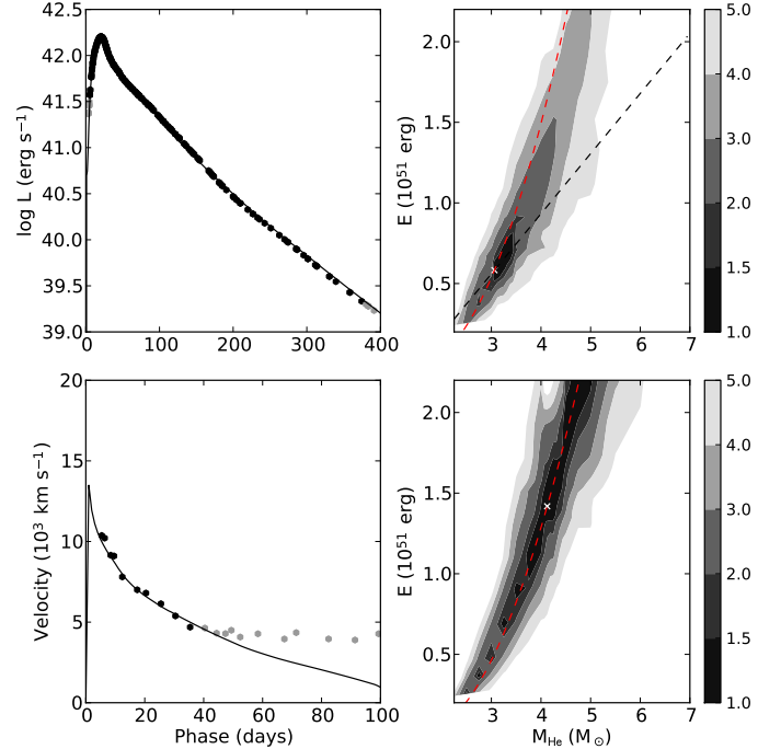
Fig. 22. Left panels: optical-to-MIR pseudo-bolometric lightcurve (upper left panel) and photospheric velocities (lower left panel) for the best-fit model (solid line) compared to observations (circles), where the photospheric velocities have been estimated from the absorption minimum of the Fe II 5169 Å line. Observations not included in the fit are shown in grey. Right panels: contour plots showing the (grey-scale coded) standard deviation in the fit, normalized to that of the best-fit model, projected onto the E - M_{\text{He}} plane for the case where the photospheric velocities were used (upper right panel) and not used (lower right panel). We also show the constraints M_{\text{ej}}/E = \text{const.} (blue line) and M_{\text{ej}}^2/E = \text{const.} (red line) provided by the photospheric velocities and the bolometric lightcurve, respectively (E15).
