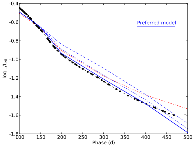
Fig. 16. Observed (black circles) and J14 model optical pseudo-bolometric lightcurves between days 100 and 500 normalized to the radioactive decay chain luminosity of 0.075 M_{\odot} of ^{56}\text{Ni} . The preferred model (12F, blue solid line), model 12C (blue short-dashed line) and model 12E (blue long-dashed line), which differ only in the optical depth (12F, 0.44; 12C, 0.25; 12E, 0) and temperature of the dust, are shown together with model 12B (red short-dashed line), which differs from model 12C only in the positron trapping (12C, local; 12B, non-local).
