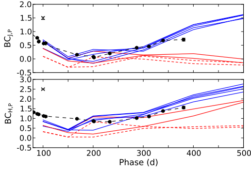
Fig. 19. Observed (black circles) and J14 model pseudo-BCs between days 100 and 500 for the J and H bands. The model families differing in contrast factor (high, solid; low, short-dashed) and positron trapping (local, blue; non-local, red) are shown. 17 M_{\odot} and medium mixing models are not shown. The error bars arising from the extinction are marked in the upper left or right corner.
