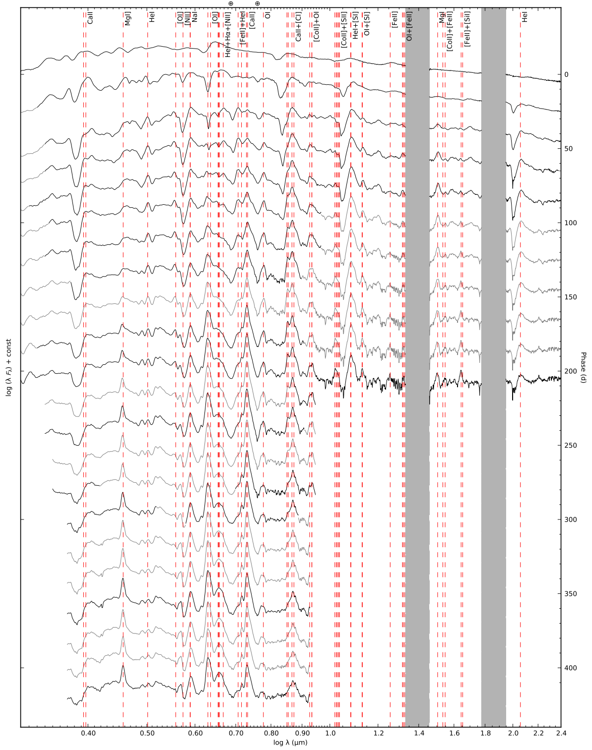
Fig. 8. Optical and NIR (interpolated) spectral evolution between days 5 and 425 for SN 2011dh with a 20-day sampling, where most of the lines identified in J14 have been marked with red dashed lines. Telluric absorption bands are marked with a \oplus symbol in the optical and are shown as grey regions in the NIR.
