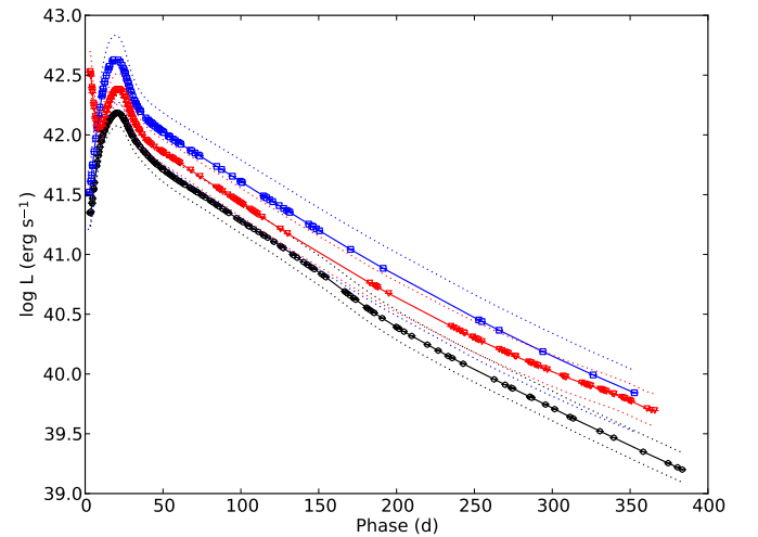
Fig. 3. Optical-to-NIR pseudo-bolometric lightcurve before day 400 for SNe 2011dh (black circles and solid line), 1993J (red triangles and solid line), and 2008ax (blue squares and solid line). The upper and lower error bars for the systematic error arising from extinction and distance (dotted lines) are also shown.
