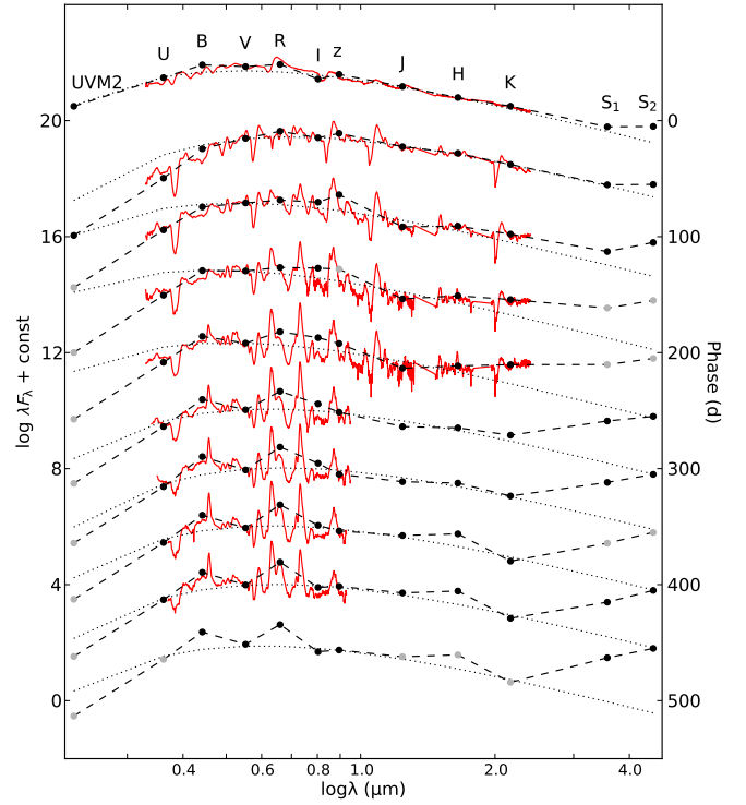
Fig. 6. Evolution of the SED (black dots and dashed lines) before day 500, overplotted with blackbody fits to the V , I , J , H , and K photometry (black dotted lines) and the observed (interpolated; Sect. 3.1) spectra (red solid lines). Fluxes based on extrapolations or interpolations over more than 25 days are shown in shaded colour.
