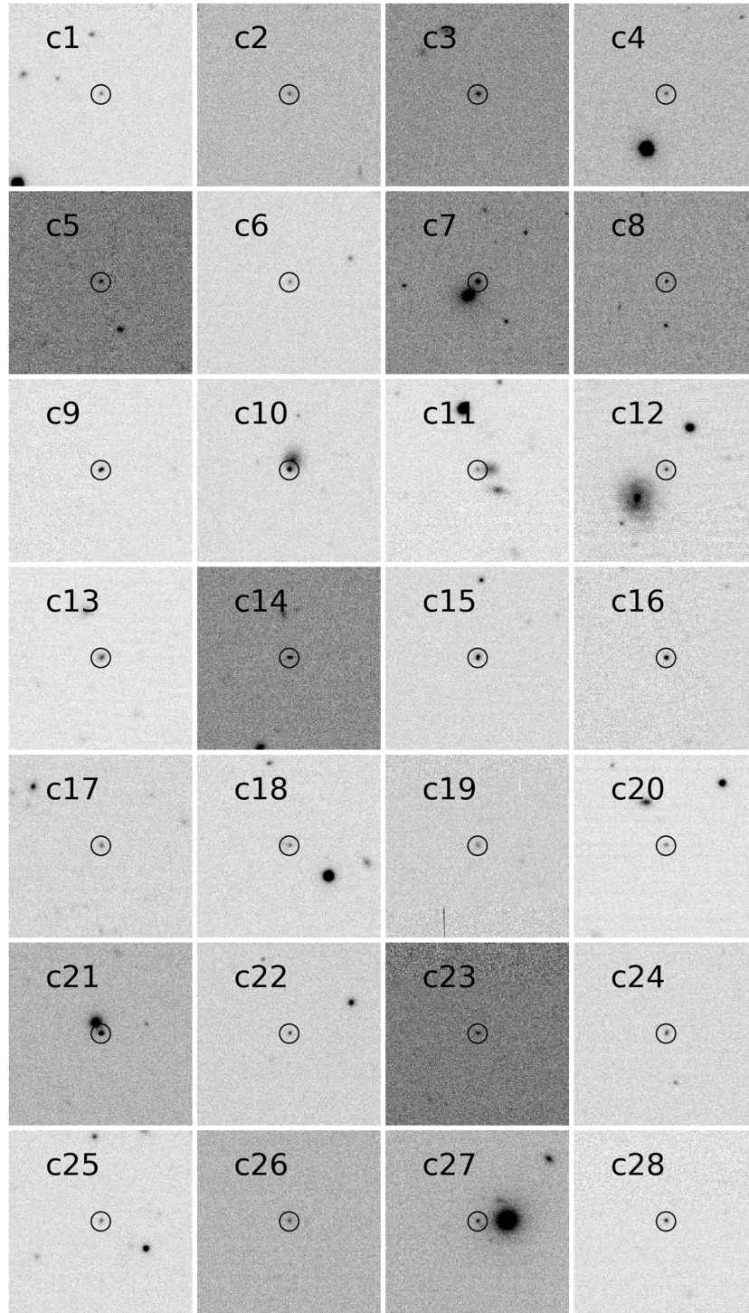
Figure B1. First 28 transient candidates found with the VST in 99 \text{ deg}^2 covering the GW170814 error area. Each image has a size of 1 \text{ arcmin} \times 1 \text{ arcmin} and is extracted from the original images at the epoch of the brightest magnitude.
