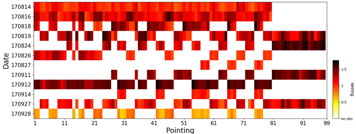
Figure 2. Overview of the survey monitoring progress. On ordinates are indicated months and days. On abscissa the VST pointings of 1 \times 1 \text{ deg}^2 . The colour indicates the seeing achieved for each specific pointing. Please refer to Table 2 to see the way nights are grouped for each epoch.
