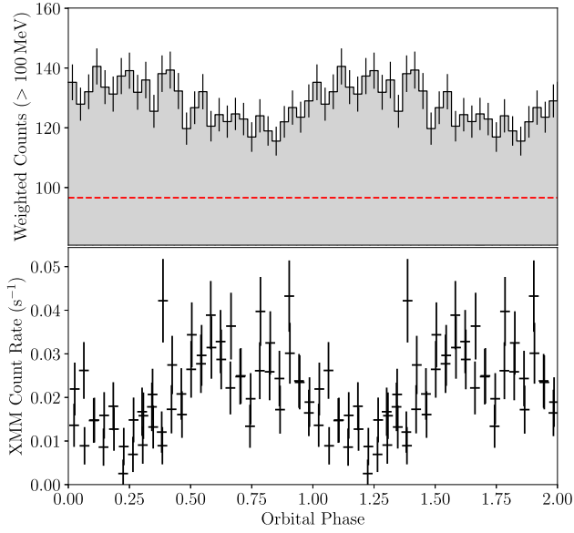
Figure 3. Orbital light curves of J2039 from XMM-Newton (lower panel) and Fermi -LAT (upper panel) observations. Data have been folded using the pulsar timing ephemeris from Section 3.2. The dashed red horizontal line on the gamma-ray light curve indicates the expected background level computed from the distribution of photon weights.
