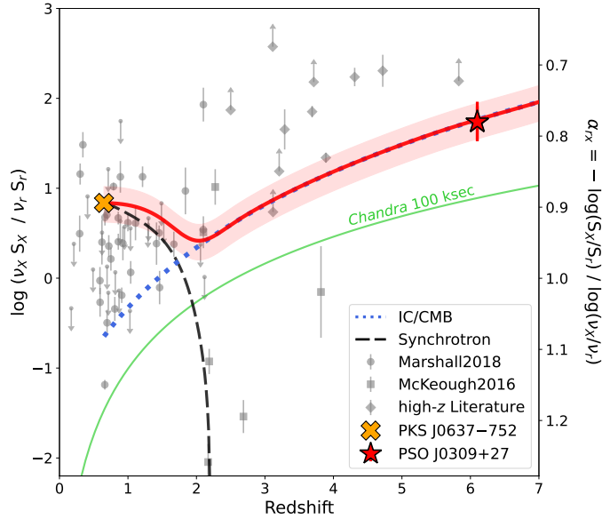
Fig. 6. X-ray-to-radio ratios (and \alpha_{\text{rx}} ) of the extended jets observed by Chandra reported in the literature. The data are from: Marshall et al. (2018), circles at z \leq 2 ; McKeough et al. (2016), squares at 2 \leq z \leq 4.7 (given by the sum of their ‘detected’ components); Siemiginowska et al. (2003), Cheung et al. (2006), Simionescu et al. (2016), Schwartz et al. (2020), Worrall et al. (2020), Snios et al. (2021); and Connor et al. (2021), diamonds at z \geq 3 . If the same object is reported in more than one work, we consider the most recent. PSO J0309+27 ( z = 6.1 ) is represented by a red star and PKS J0637–752 ( z = 0.65 ) by an orange cross. The solid red line connecting the two sources is the evolution of the X-ray-to-radio ratio as a function of redshift based on the model reported in Fig. 5, where the extended X-ray emission is given by the sum of a synchrotron (dashed black line) and an IC/CMB component (dotted blue line). The solid green line represents the limit above which an extended X-ray jet with the same radio luminosity as the one found in PSO J0309+27 can be observed with a 100 ksec Chandra exposure.
