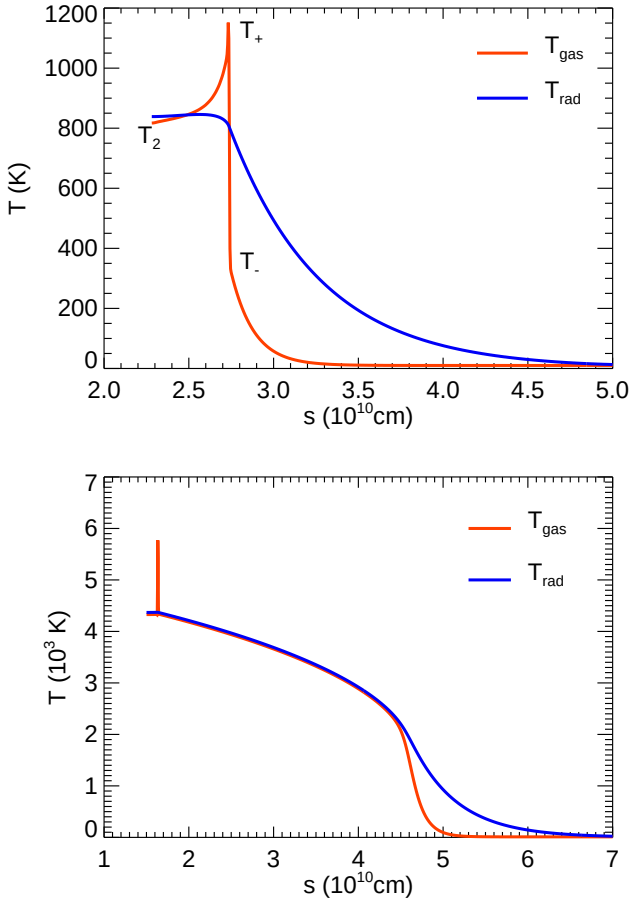
Fig. 3. Gas temperature (red) and radiation temperature (blue) vs. s = z - vt for the sub- (top panel) and supercritical (bottom panel) shocks. The subcritical shock is shown at time t = 3.8 \times 10^4 s and the supercritical shock at t = 7.5 \times 10^3 s.
