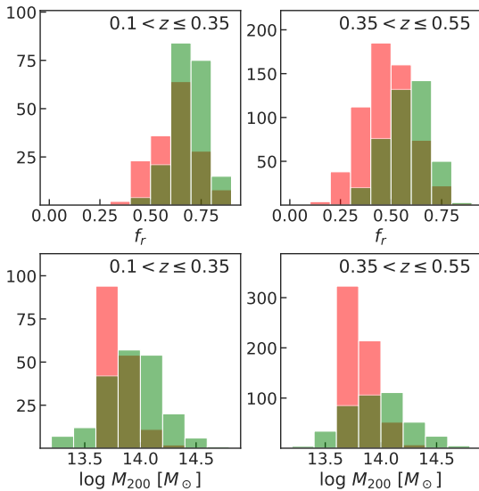
Figure 10. Distribution in fraction of red galaxies ( f_r ) and mass (from AMICO) in two redshift bins for the matched (green) and unmatched (red) clusters from the KiDS-AMICO vs. redMaPPer catalogues. A cut on mass, \log M_{200} > 13.5 M_{\odot} , was applied to unmatched clusters.
