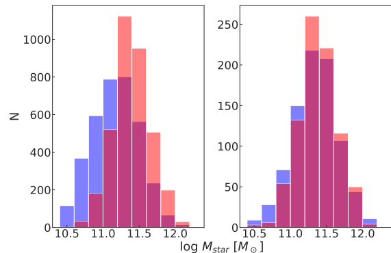
Figure 15. Distribution of BCG stellar masses in KiDS-AMICO (blue), the Illustris TNG300-1 sample (light red). In the left panel the Illustris TNG300-1 simulations are matched in cluster mass and redshift to the KiDS-AMICO subsample with measured BCG stellar mass; in the right panel a further selection of clusters with \Delta M_{1,2} > 1 is done.
