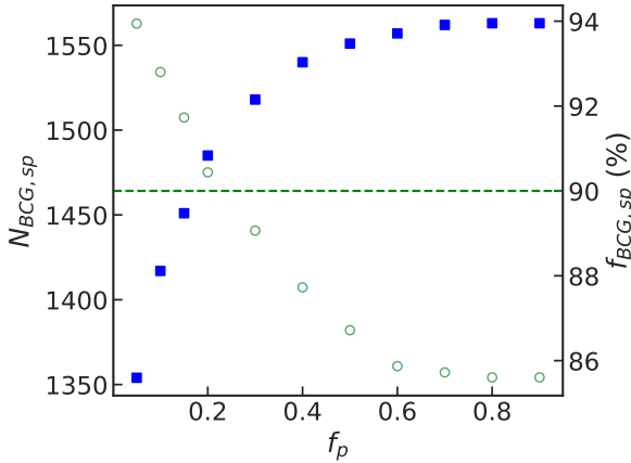
Figure 2. The plot displays, for different values of f_p : filled squares - the number of BCGs with spectroscopic redshifts, left axis); empty circles - the fraction of BCGs with cluster redshifts in agreement with spectroscopic redshifts as defined in the text ( f_{\text{BCG,sp}} , right axis). The dashed line is the threshold fraction adopted to select the optimal values of f_p .
