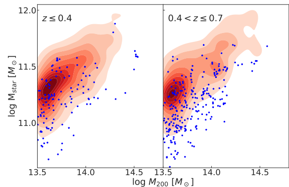
Figure 16. BCG stellar masses vs. cluster masses in the Illustris TNG300-1 sample: red contours display the distribution for red BCGs, values for blue BCGs are plotted as blue stars.
