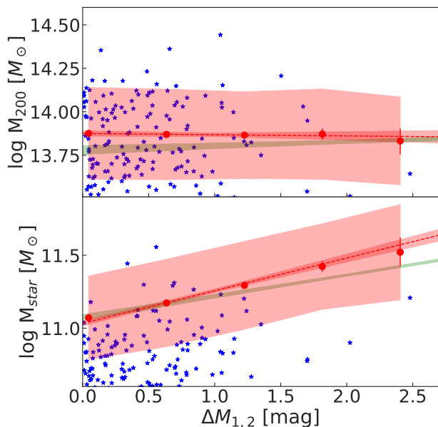
Figure 14. Total cluster mass (top panel) and stellar mass (bottom) as a function of the magnitude gap. The wider area (light red) shows the 1\text{-}\sigma scatter for observed values, whose bootstrapped average values and error bars are plotted as red circles. Blue BCGs are displayed as blue stars. The fits derived from the Illustris TNG300-1 simulations are marked in green. Shaded areas display 95% confidence intervals.
