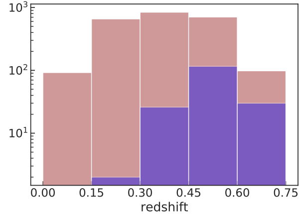
Figure 11. Redshift distribution of red and blue BCGs.
