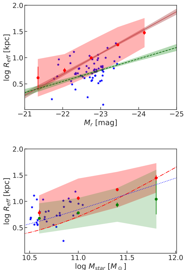
Figure 12. Top: size-luminosity distribution in BCGs. The wide area (light red) shows the 1\text{-}\sigma scatter for observed values, whose bootstrapped average values and error bars, and linear fits, are plotted in red. Values for blue BCGs are displayed as blue stars. The linear fits for galaxies with a low membership probability are displayed in green; shaded areas display 95% confidence intervals. Bottom: the size-stellar mass is displayed for BCGs with 0.3 < z < 0.5 (same symbols as above) and compared with the fits at z \sim 0.4 derived by Roy et al. (2018) for spheroid (dashed-dotted red) and disc (dotted blue) galaxies. The wide green area shows the 1\text{-}\sigma scatter for low membership probability galaxies.
