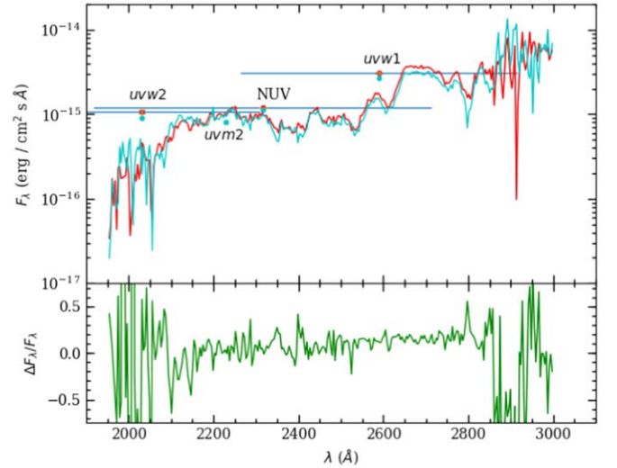
Figure 6. Top: comparisons of GALEX NUV spectra for the binary WOCS 11028 (red) and likely main-sequence star WOCS 6018 (cyan). Photometry from GALEX (NUV filter) and Swift/UVOT is shown as points, with the approximate widths of the filters shown as horizontal bars. Bottom: fractional difference between GALEX spectra of WOCS 11028 and WOCS 6018.
