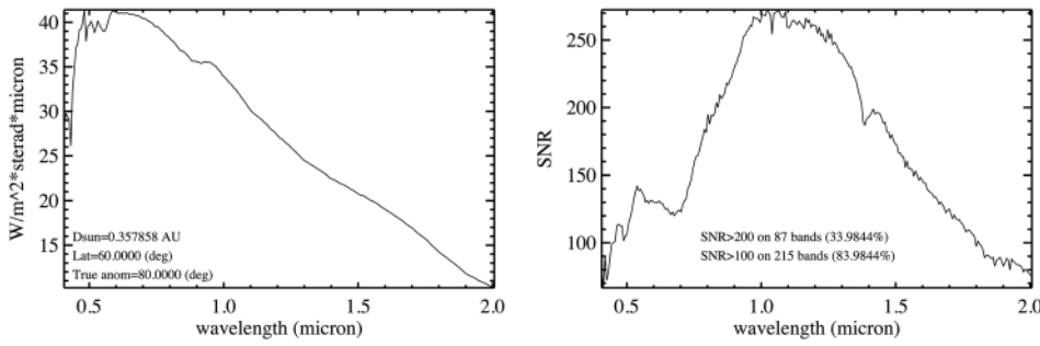
FIG. 16. Expected spectral radiance for Mercury low albedo terrain (left panel) and instrumental SNR (right panel) for case 4 with t_{\text{exp}} = 30 ms.
