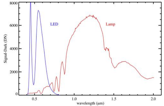
FIG. 17. VIHI internal calibration unit reference spectral signals from LED and lamp at boresight ( s = 128 ).
