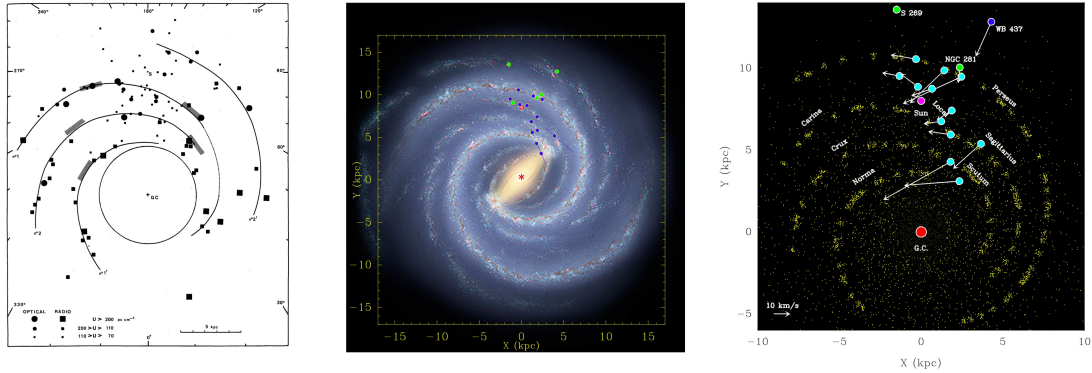
Figure 2: Left: The Georgelin & Georgelin (1976) model, based on HII region recombination line velocities and stellar luminosity distances. Middle: An artists impression of the Milky Way, created from the 2-arm barred spiral model of (56) and scaled to fit the trigonometric parallaxes of 12.2 GHz \text{CH}_3\text{OH} masers (57). Right: The (51) refinement of the Georgelin & Georgelin model with overlaid positions and peculiar velocities of \text{H}_2\text{O} masers observed with VERA and 12.2 GHz \text{CH}_3\text{OH} masers observed with the VLBA. Note the complete absence of any trigonometric maser parallaxes in the Southern Galactic Plane (i.e. the Norma, Crux & Carina arms).
