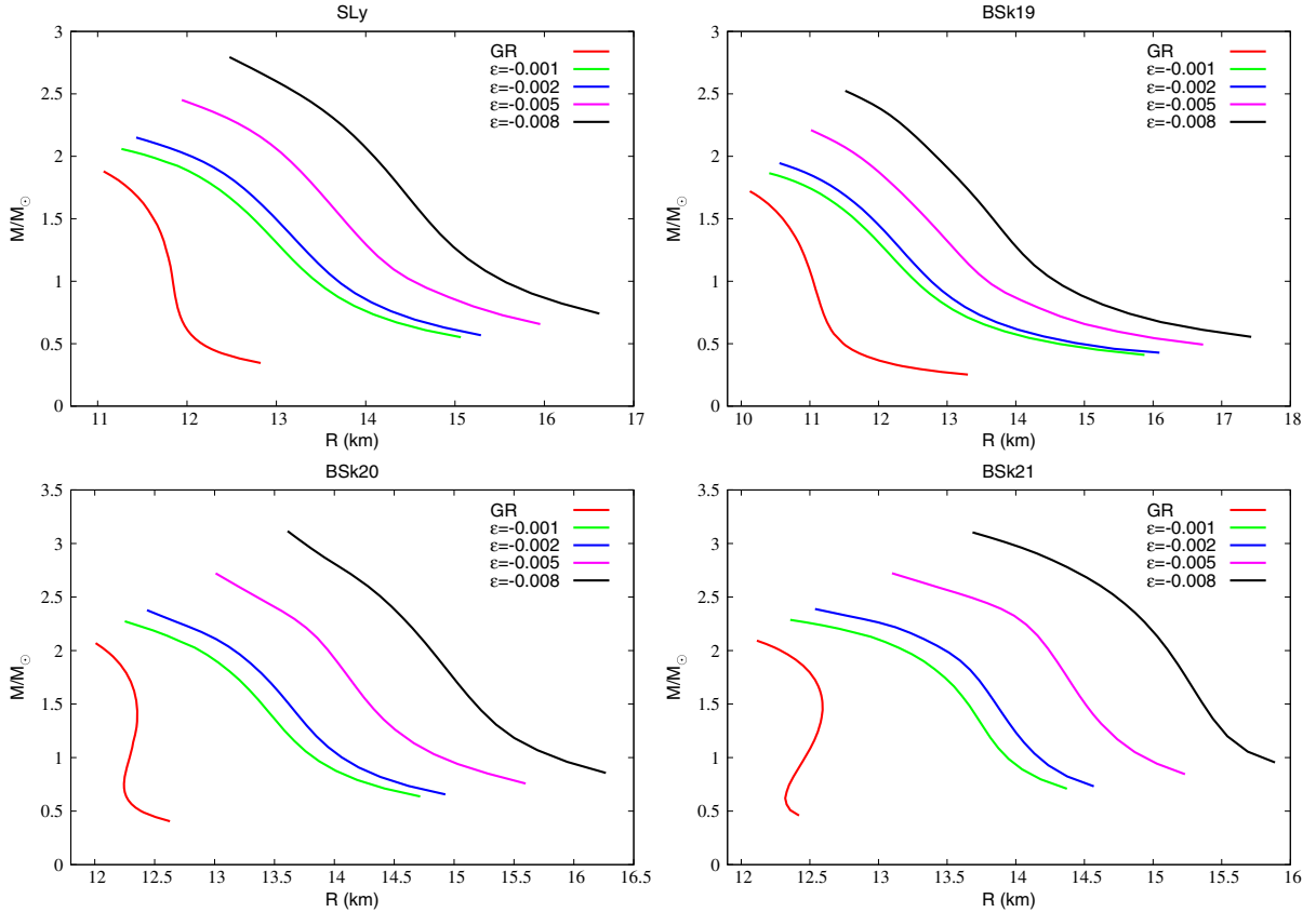
FIG. 6. M - R diagrams for f(R) given in Eq. (15) with four EoS and different values of \epsilon . The classical TOV corresponding to \epsilon = 0 is also reported.
