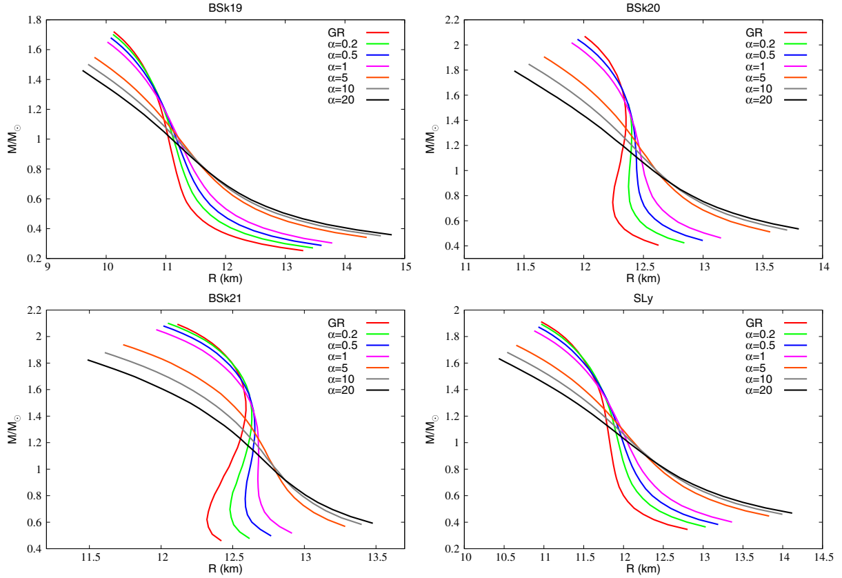
FIG. 2. M - \mathcal{R} diagrams for different EoSs (labeled in the top of each panel) and quadratic form f(R) = R + \alpha R^2 . For each EoS the maximal central density is determined by the condition \rho_c - 3p > 0 (see text). The classical TOV solution is also reported. The values of \alpha are in the modulus.
