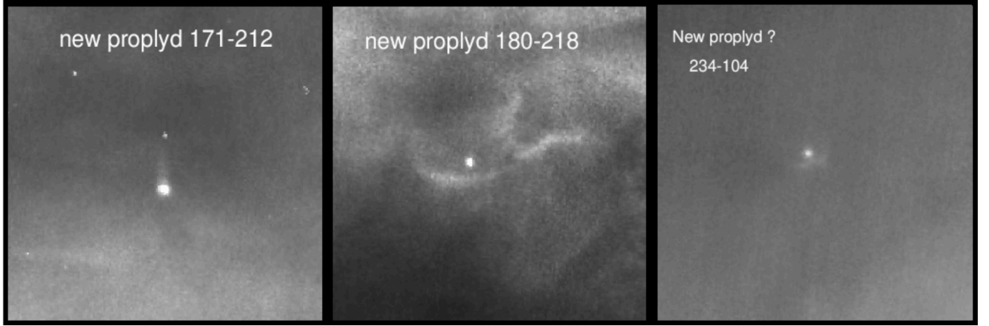
Fig. C.13. Zoom on the 3 new bright proplyds identified in the F187N NIRCам image north-east of the Trapezium stars (module A): 171-212, 180-218 and 234-104. They have faint cusps and only one shows a tail in Pa \alpha , that is proplyd 171-212. The tiles are 5'' \times 5'' with north up and east to the left.
