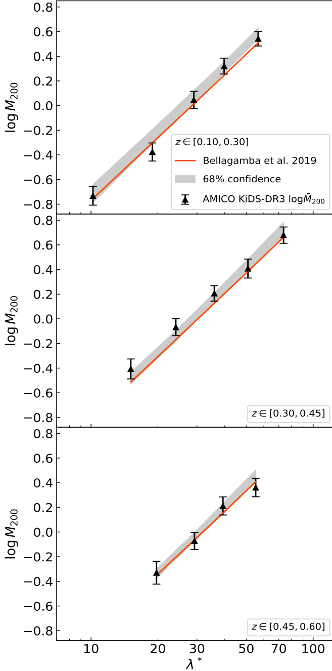
Fig. 2. Logarithm of the masses in units of (10^{14} M_{\odot} h^{-1}) , \log \bar{M}_{200} , from the AMICO KiDS-DR3 cluster catalogue as a function of the intrinsic richness \lambda^* , in the redshift bins z \in [0.10, 0.30] , z \in [0.30, 0.45] , and z \in [0.45, 0.60] , from top to bottom. The black triangles represent the mean values of \log \bar{M}_{200} , given by the mean of the marginalised posterior obtained in the weak lensing analysis, while the error bars are given by 1\sigma of the posterior distribution. The orange lines represent the median scaling relation obtained by modelling only \log \bar{M}_{200} , following the procedure described in Bellagamba et al. (2019). The grey bands represent the 68% confidence level derived from the multivariate posterior of all the free parameters considered in the cosmological analysis described in Sect. 3.
