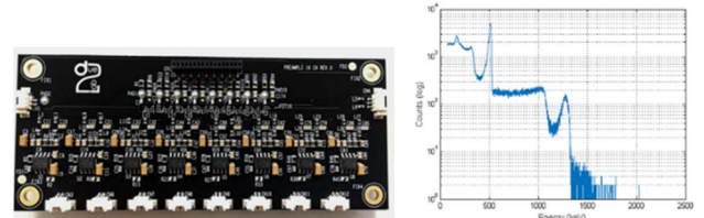
Figure 8: the 16 channel CSP board (left); the measured spectrum of a ^{22}\text{Na} source (right) obtained using a hemispheric ( 0.5 \text{ cm}^3 ) CZT detector polarized at -1100 V.
