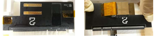
Figure 7. The 3D CZT sensor support: (left) anode side; (right) cathode side with the 10 Au lines on Kapton still folded, to be connected'.
