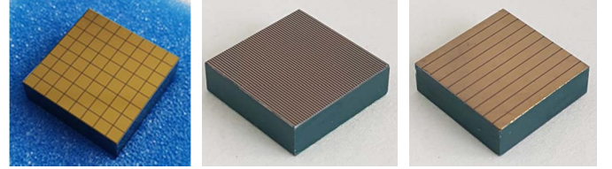
Figure 4. (left) Original CZT crystal tile; (center) final anode side configuration; (right) final cathode side segmentation.
