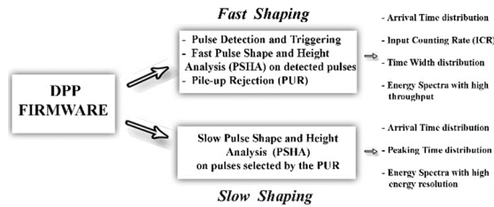
Figure 10. The DPP system firmware pipelines, with main operations and the output data.
