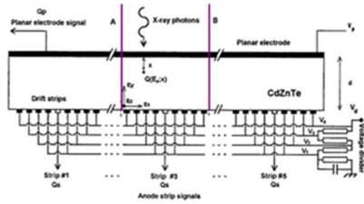
Figure 1. A typical anodic drift strip configuration.
