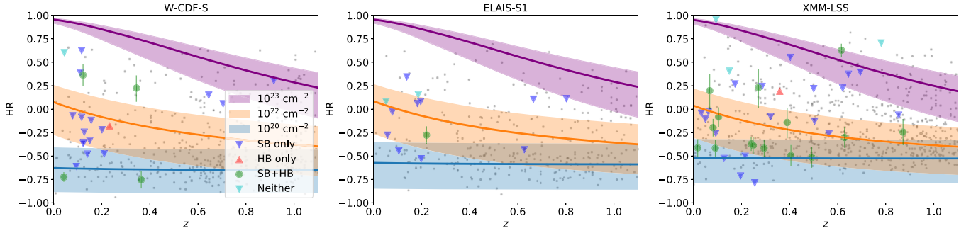
Figure 8. HR vs. z in W-CDF-S (left), ELAIS-S1 (middle), and XMM-LSS (right). The background gray points are general XMM-SERVS sources detected in both the SB and HB. The large colored points are our active dwarf galaxies, and their legend in the left panel indicates their detection status in the SB and HB. The blue downward triangles, which are detected in the SB but not the HB, represent 95% HR upper limits; while the red upward triangles, which are detected in the HB but not the SB, are 95% HR lower limits. Green points with error bars represent the median HR values with 1\sigma uncertainties for sources detected in both bands. The cyan downward triangles are the 95% HR upper limits for sources only detected in the FB. The shaded regions are the expected relations for redshifted absorbed power-laws, whose photon indices vary between 1.4 and 2.6, with several different N_{\text{H}} values, as labeled in the legend. Their corresponding solid curves mark the case when the photon index is 1.8. Our sample is generally below the N_{\text{H}} = 10^{23} \text{ cm}^{-2} region and thus not heavily obscured in X-rays.
