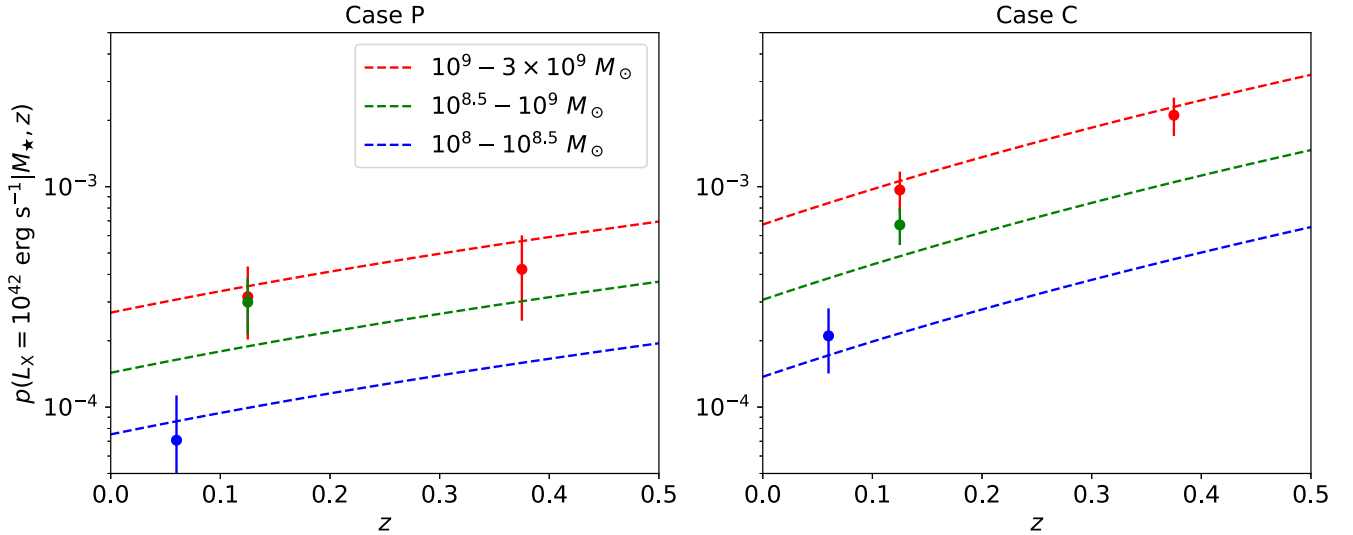
Figure 13. Our fitted p(L_X|M_*, z) model (dashed lines) and the corresponding four binned estimators based on our data (points with error bars) as functions of z . The model and binned estimators are both evaluated at L_X = 10^{42} \text{ erg s}^{-1} and the M_* bin centers. The left and right panels are for Cases P and C, respectively. Our model is consistent with the binned estimators.
