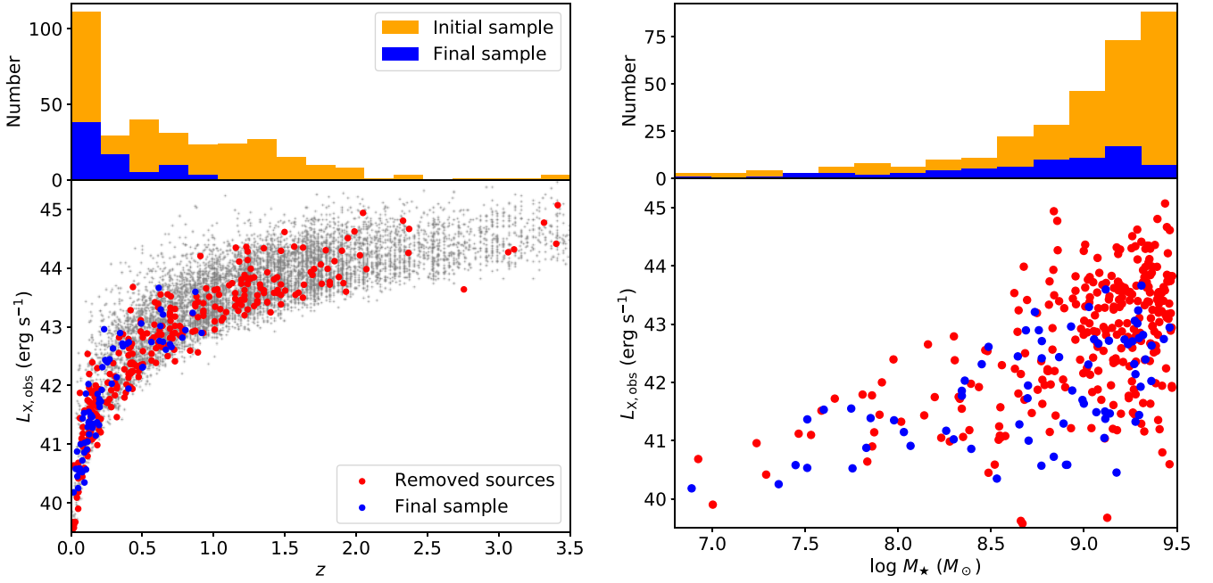
Figure 6. Left: the z – L_{X, \text{obs}} plane. The gray small points are all the XMM-SERVS sources. The blue points are our final active dwarf-galaxy sample, and the red ones are those removed from the initial sample. The top histograms show the redshift distributions of the initial (orange) and final (blue) samples. Right: similar to the left panel but for the M_* – L_{X, \text{obs}} plane, and its top histograms are for the M_* distributions. Our final sample size is much smaller than the initial sample size, highlighting the overall challenges of reliably selecting distant active dwarf galaxies. Selection biases inevitably exist, especially at high redshifts.
