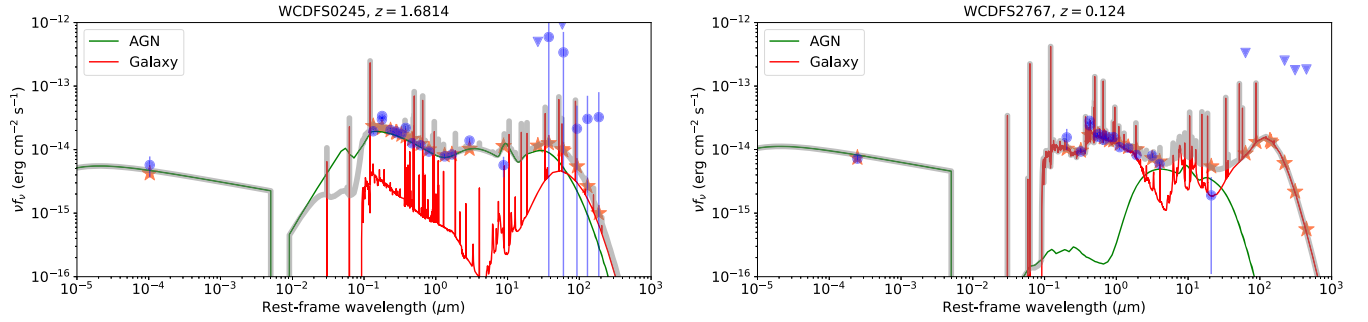
Figure 3. Example rest-frame SEDs from Z22 of high-redshift X-ray-detected dwarf galaxies with M_\star < 3 \times 10^9 M_\odot (left) and bona fide active dwarf galaxies (right). The source XIDs and redshifts are listed as the panel titles. The blue points and downward triangles are the observed photometry and upper limits, respectively. The orange stars are the best-fit modeled photometry in the given bands, and the thick gray lines represent the best-fit models. The SEDs are decomposed into AGN components (green) and galaxy components (red). In contrast to the right panel, the AGN component in the left panel dominates the optical-to-NIR SED, and thus the host M_\star cannot be measured reliably.
