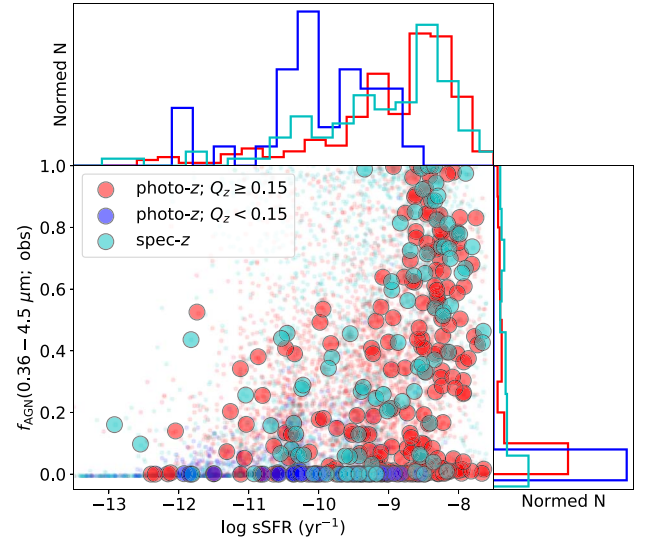
Figure 2. \log \text{sSFR} vs. f_{\text{AGN}}(0.36-4.5 \mu\text{m}; \text{obs}) for all the XMM-SERVS sources. Galaxies with cataloged M_* < 3 \times 10^9 M_\odot are marked with large points. Distributions of \log \text{sSFR} and f_{\text{AGN}}(0.36-4.5 \mu\text{m}; \text{obs}) are shown in the top and right panels, respectively. Sources whose redshifts are photo- z s with Q_z \geq 0.15 (i.e., the large red points) are removed from our sample. The photo- z quality cut only retains sources with small sSFR and near-zero f_{\text{AGN}}(0.36-4.5 \mu\text{m}; \text{obs}) .
