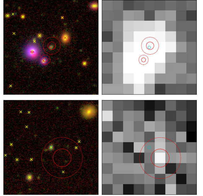
Figure 5. The optical (left) and XMM-Newton 0.2–12 keV (right) images of example sources failing the X-ray excess criterion. The top panels are for \text{XID} = \text{WCD4029} , and the bottom ones are for \text{XID} = \text{WCD4098} . The three-color optical images are generated from g -band (blue), i -band (green), and z -band (red) images from Ni et al. (2019; top). The red and yellow crosses mark AGNs and non-AGNs in Z22, respectively. The cyan circles are centered at the dwarf targets with radii of 0.5'' . The red solid and dashed circles represent 68% and 99.73% X-ray positional uncertainties, respectively, for the X-ray sources.
