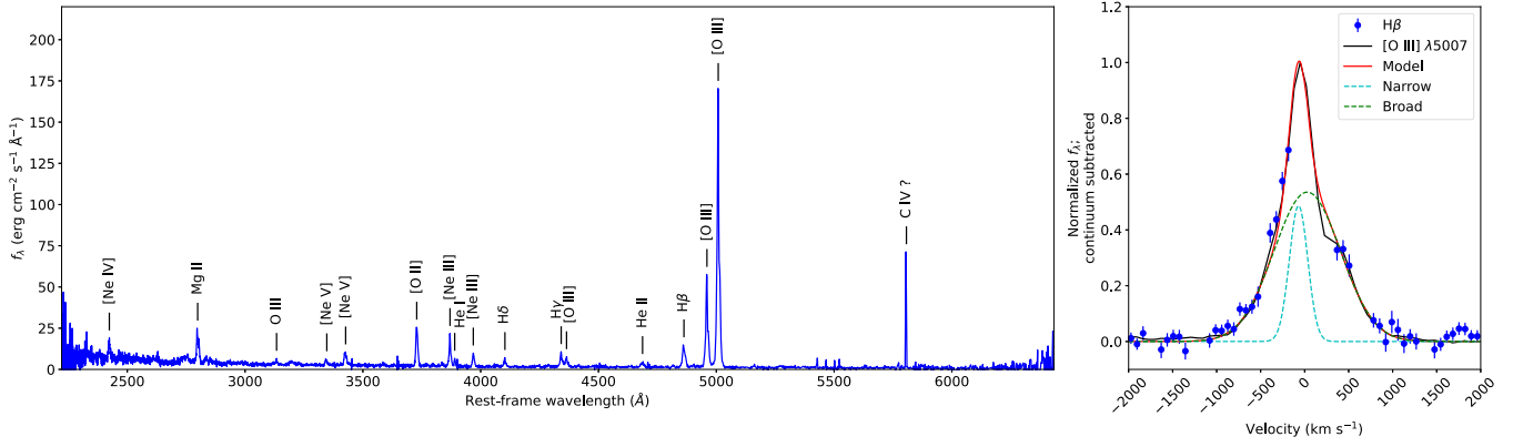
Figure 20. Left: SDSS rest-frame spectrum of XMM02399 after correcting for Galactic extinction. Apparent emission lines are marked explicitly. The C IV \lambda 5808 line is uncertain due to large uncertainties in the corresponding pixels. Right: normalized H \beta and [O III] \lambda 5007 profiles in the velocity space. Negative velocity indicates blueshift. H \beta is shown as points with error bars, while [O III] \lambda 5007 is shown as the black solid line. The best-fit model for [O III] \lambda 5007 is shown as the red solid line, whose narrow and broad components are plotted as the cyan and green-dashed lines, respectively. H \beta is consistent with the [O III] \lambda 5007 profile.
