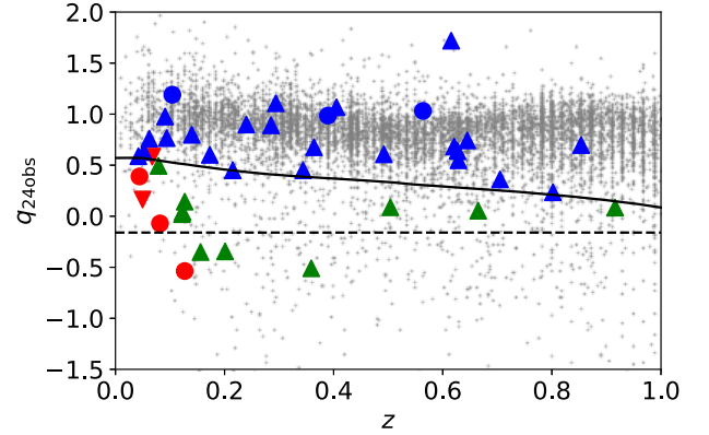
Figure 9. q_{24\text{obs}} vs. z . The black solid and dashed lines are the q_{24\text{obs}} thresholds for radio-excess AGNs in Bonzini et al. (2013) and Zhu et al. (2023), respectively. The colored points or triangles mark our active dwarf galaxies that have radio coverage and are detected in at least one of the 24\mu\text{m} and 1.4 GHz bands. The points are those detected in both bands and thus have q_{24\text{obs}} values, the downward triangles represent q_{24\text{obs}} upper limits for sources only detected in the radio, and the upward triangles are q_{24\text{obs}} lower limits for sources only detected at 24\mu\text{m} . Sources are colored in red if they are classified as radio-excess AGNs according to the criterion in Bonzini et al. (2013), blue if they are above the black solid line (i.e., not radio-excess AGNs), and green if unable to be classified. The background gray points are general radio sources in our fields (Zhu et al. 2023). Their photo- z s are mildly quantized because these photo- z s (same as those in Z22) are derived at a series of redshift grid points. This grid has a bin size of \delta z/(1+z) < 0.01 and is thus sufficiently dense to avoid noticeable biases. Only a limited fraction of our sources are radio-excess AGNs.
