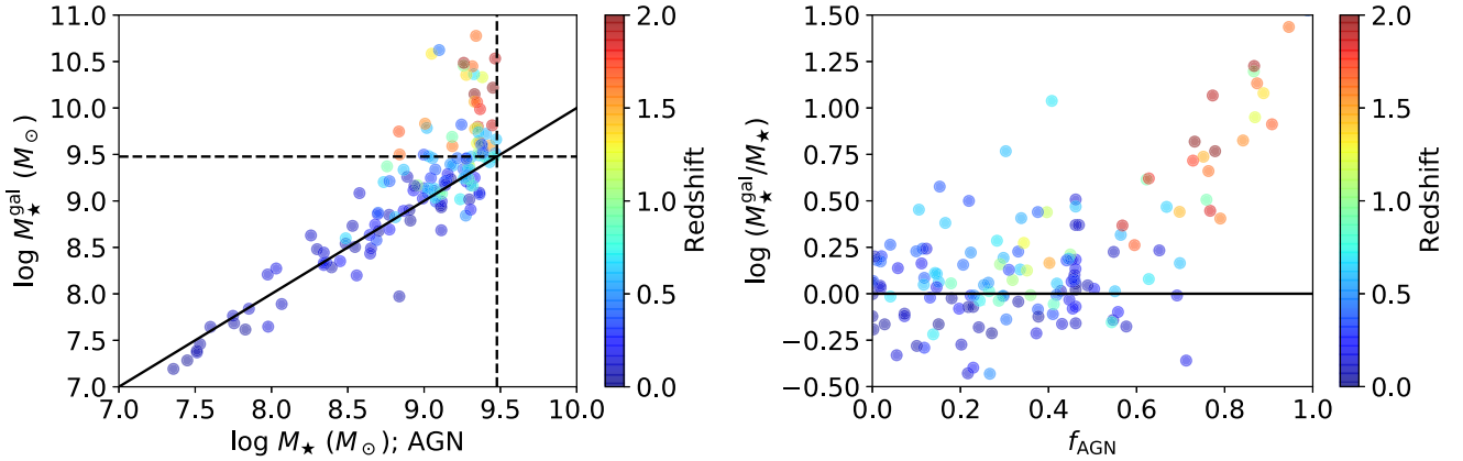
Figure 4. Left: comparison between M_\star^{\text{gal}} and the adopted AGN-template-based M_\star values, color coded by redshift. The black solid line represents a one-to-one relationship, and the black-dashed lines are our adopted mass threshold ( 3 \times 10^9 M_\odot ) for both M_\star^{\text{gal}} and M_\star . Sources above M_\star^{\text{gal}} = 3 \times 10^9 M_\odot are not considered. Right: difference between M_\star^{\text{gal}} and M_\star vs. f_{\text{AGN}}(\text{IR}) , color coded by the redshift. The black solid line represents zero difference. The difference between M_\star^{\text{gal}} and M_\star generally increases with f_{\text{AGN}}(\text{IR}) , and high-redshift sources tend to have larger f_{\text{AGN}}(\text{IR}) and often exceed the threshold of M_\star^{\text{gal}} .
