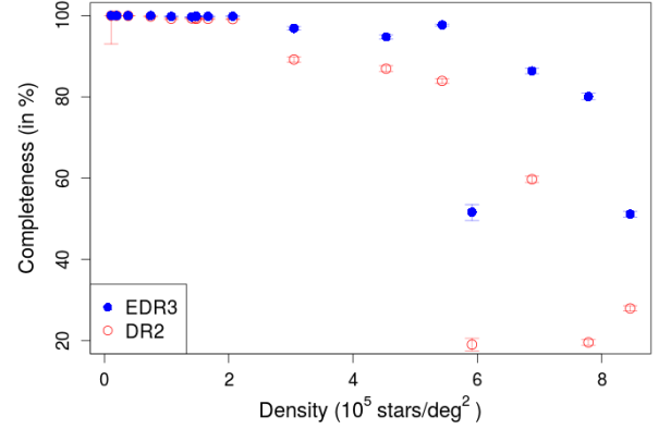
Fig. 6. Improvement of the Gaia completeness at G=20 mag versus some OGLE fields of different stellar densities from Gaia DR2 (red) to Gaia EDR3 (blue).
