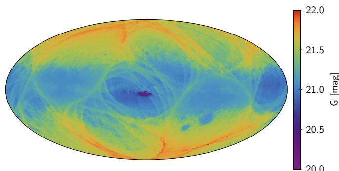
Fig. 2. Map in Galactic coordinates of the 99th percentile of the G magnitude at healpix level 5, i.e. in 3.36^\circ pixels.
