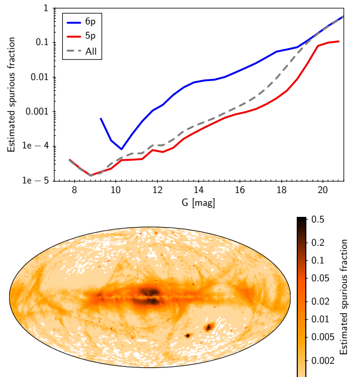
Fig. 13. Estimated fraction of spurious solutions for sources where the formal uncertainty is at least five times smaller than the parallax. Top : The fraction by G for the whole catalogue (dashed line) as well as separately for 5p (lower, red line) and 6p (upper, blue line) solutions. Bottom : Skymap of the fraction for the whole catalogue in Galactic coordinates.
