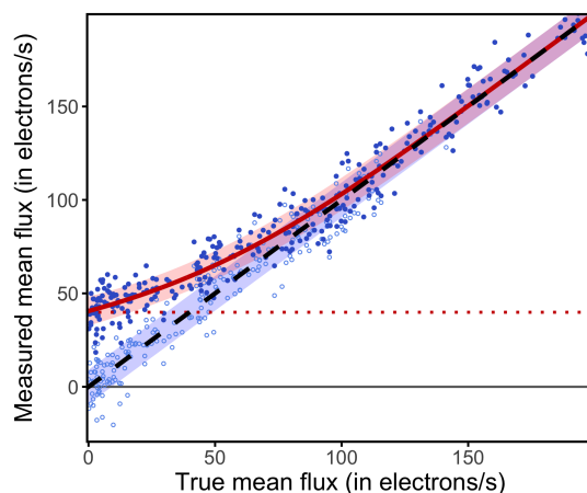
Fig. 29. Simulated mean fluxes as a function of the true mean flux in the presence of the 1 \text{ e}^- \text{ s}^{-1} threshold (dark filled symbols) and without (light open symbols). The mean and the 1\sigma confidence intervals are shown as lines and shaded regions. The dotted line indicates the lower bound of the mean in the presence of the threshold.
