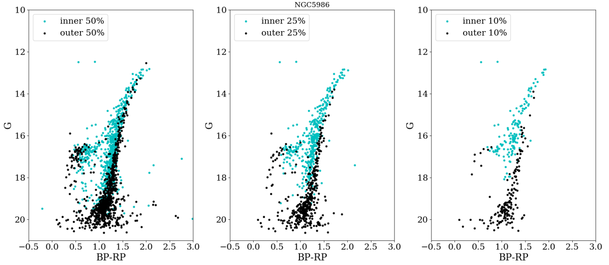
Fig. 38. Colour magnitude diagram in the inner (blue) and outer (black) regions of NGC 5986 in three different areas: inner 50% and outer 50% (left); inner 25% and outer 25% (centre); and inner 10% and outer 10% (right).
