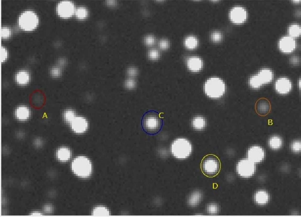
Figure 19: FoV = 0.15'' \times 0.12'' The objects circled have been analysed using SExtractor (Bertin & Arnouts, 1996, A&AS 117, 393). They are: a) Star of K magnitude 30.51 (S/N=12). b) Star of K magnitude 29.18 detected with S/N=45. c) Star of K magnitude 27.74 detected with S/N=168. d) Star of K magnitude 27.22 detected with S/N=271.
