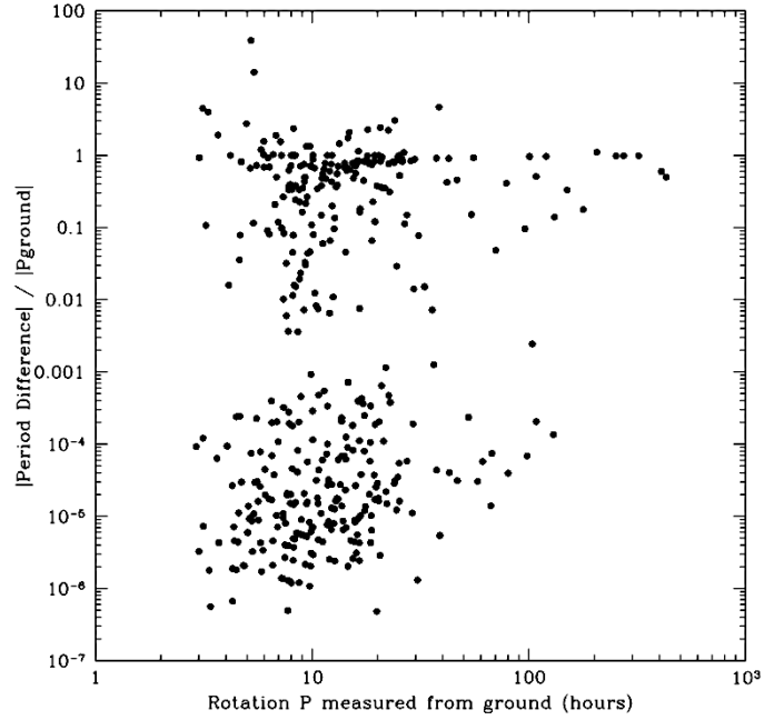
Fig. 24. Relative difference between the absolute value of the difference between the resulting P solution and the P value determined by ground-based observations in units of the ground-based P value for each object of the considered sample.
