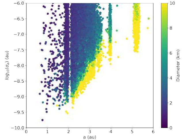
Fig. 20. Semi-major axis (au) vs. log 10 of the semi-major axis uncertainty (au) for the objects for which the orbit determination procedure converged during the validation process. The colour bar represents the diameter estimate for each object from JPL SBDB.
