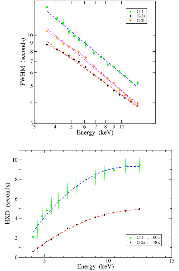
Fig. 4. Upper panel: energy scaling of the pulse FWHM of the bursts in the pointings G-1 (green squares), G-2a (black circles), and G-2b (orange diamonds). Error bars of the G-2a data set are smaller than the symbols. Power law best fits for all data sets are given by dashed lines, while the broken power-law best fits for G-2a and G-2b data are given by dash-dotted lines. Lower panel: HXD plotted as a function of energy for the G-1 and G-2a data set; the mean recurrence times of the bursts are reported. Colour codes are as in the upper panel. The dashed lines are quadratic best fits.
