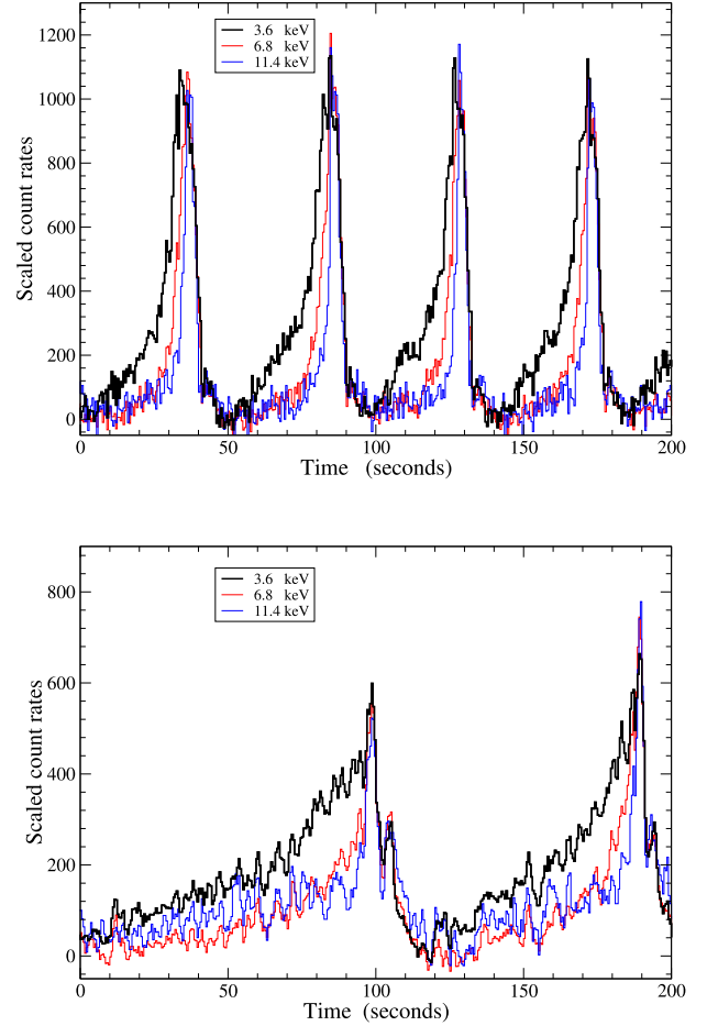
Fig. 1. Two segments of RXTE/PCA light curves of GRS 1915+105 in the \rho variability class at three energies showing the HXD phenomenon and the dependence of the pulse width, w , upon energy. Data, after the subtraction of a constant level, are scaled to obtain comparable pulse heights. Upper panel: RXTE G-2a data; lower panel: G-1 data. In the latter data set the recurrence time of the bursts was more than twice longer than that in the former one. We note in both panels the variable duration and shape of individual bursts and in the upper one the small time delay of the peak maxima, particularly in the first and in the third burst.
