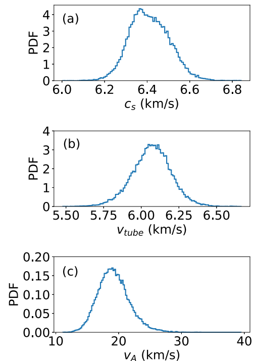
Fig. 8 Characteristic speeds inside the sunspot. Probability density function (PDF) of the main characteristic speeds inferred from a modeling based on spectropolarimetric inversions of the Fe 6173 Å spectral data within the umbra. a Sound speed in the umbra. b Tube speed in the umbra. c Alfvén speed in the umbra. Source data are provided as a Source Data file.
