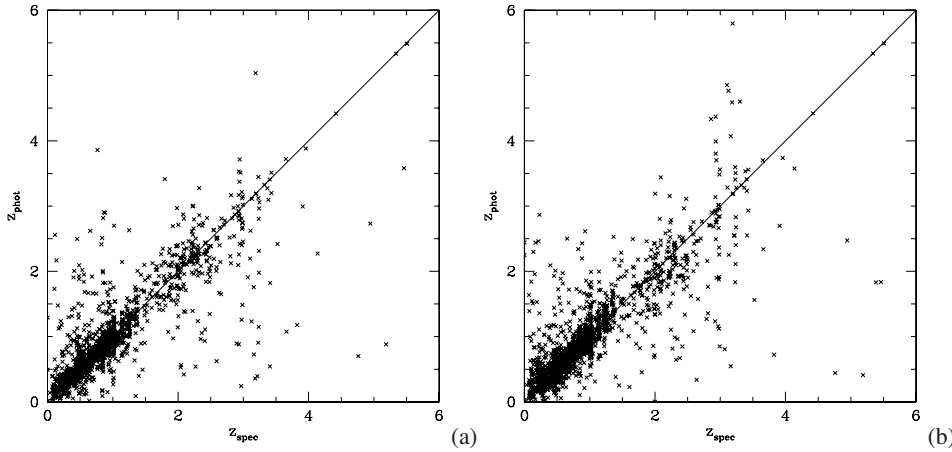
Fig. 2. Results obtained by our model and provided by the PHAT contest board in terms of direct comparison between our photometric and blind spectroscopic information. The a) panel plots the photometric vs. spectroscopic redshifts for the whole dataset using 10 photometric bands (Experiment 37). In panel b) the same but using only 14 photometric bands (Experiment 26). (Courtesy of H. Hildebrandt).
