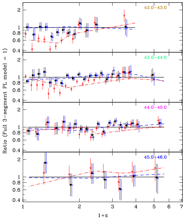
Figure 8. Comparison of best-fit models and the N_{\text{obs}}/N_{\text{mdl}} estimates in each luminosity class. The best-fit three-segment power-law models of the no-pz-PDF and \Gamma = 1.8 cases are divided by those of the full case. The N_{\text{obs}}/N_{\text{mdl}} XLFs are also divided by the full model. The data points of the no-pz-PDF and \Gamma = 1.8 cases are shifted horizontally by +0.007 and -0.007 , respectively, in \log(1+z) for display purposes. See Figure 7 for the meanings of line styles, symbols, and colors.
