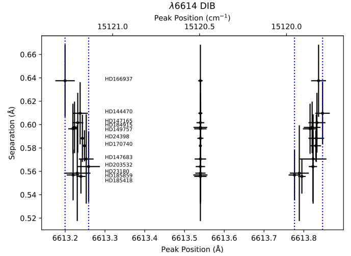
Fig. 5. Measured peak positions of the \lambda 6614 DIB in our target sightlines. Positions have been shifted such that the Q -branch lies at 6613.54 Å in all lines of sight.
