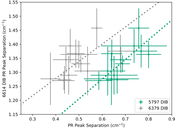
Fig. 4. P - to R -branch separation in all sightlines of the \lambda 6614 DIB (vertical axis) as a function of the separation of the \lambda 5797 (green) and 6379 (grey) DIBs on the horizontal axis (data values are listed in Table 2). The dotted lines are linear models of the data using orthogonal-distance fitting of the 6614 measurements as a function of the 5797 values (green) and 6379 values (grey).
