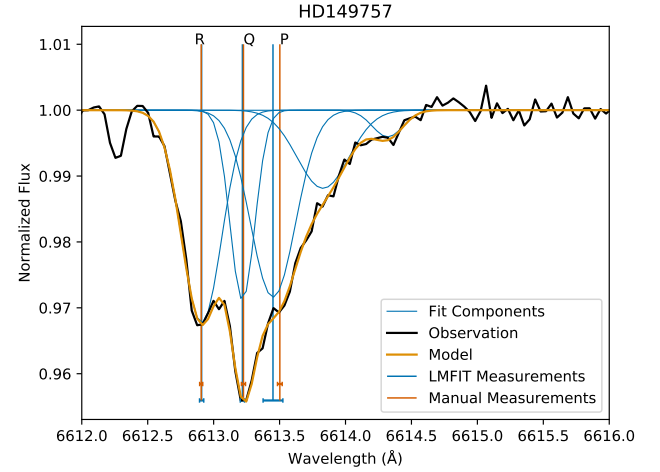
Fig. 3. Observed \lambda 6614 DIB profile toward HD 149757 (black) and the best fitting model profile (orange) composed of five individual Voigt profiles (blue). The blue vertical lines indicate the central wavelengths of the three main components from the model fit. Dark orange vertical lines indicate the peak positions determined with the alternative manual measurement process. Especially for the third peak, both positions differ from each other, and the peak position from the model fit does not correspond to the peak absorption. Uncertainties on these measurements are indicated by the error bars at the bottom of each line. The peak positions are labelled as P, Q or R branches, consistent with our rotational contour terminology.
