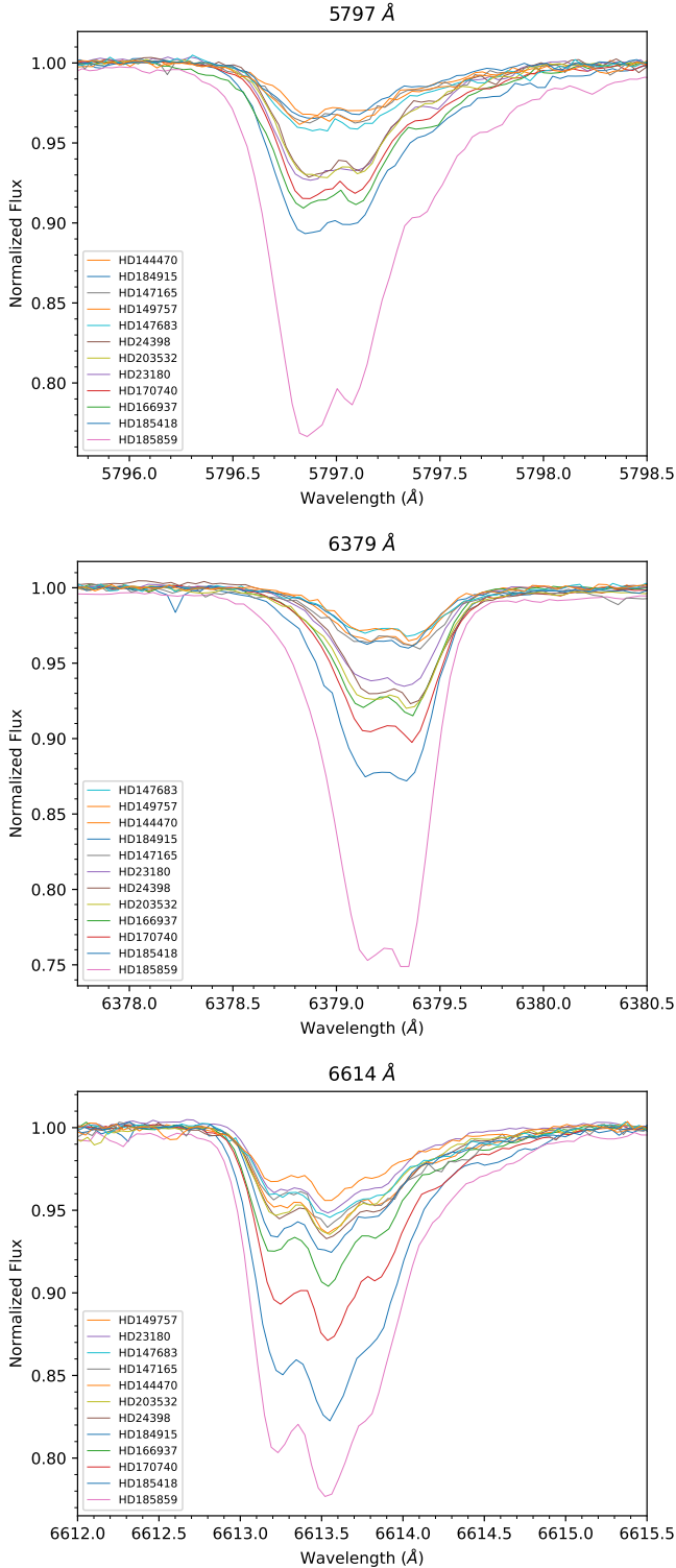
Fig. 2. Co-added observations of our sample sight lines, shifted to the interstellar rest frame for respectively the \lambda 5797 (top panel), 6379 (middle panel) and 6614 (bottom panel) DIBs.
