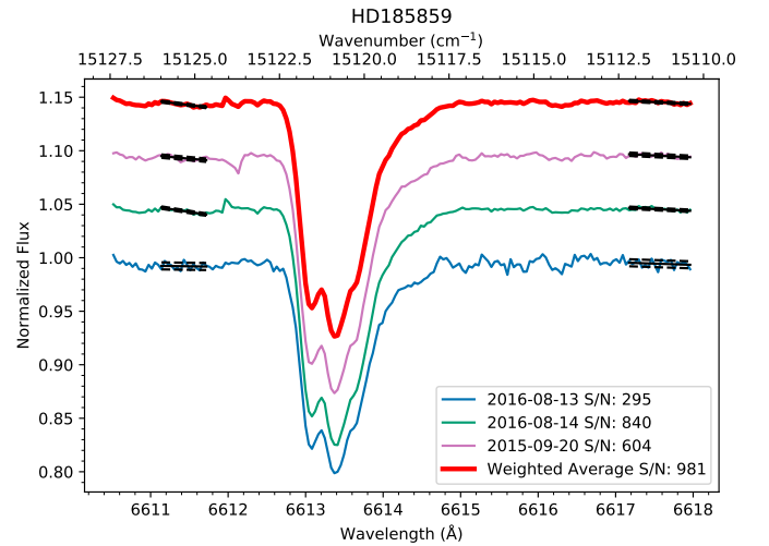
Fig. 1. All available EDIBLES observations of the \lambda 6614 DIB toward HD 185859 (thin lines), and our weighted average spectrum (thick red line). Observation dates and S/N are indicated in the legend. The S/N was estimated from the standard deviations in the regions marked in black. A vertical offset is added for clarity.
