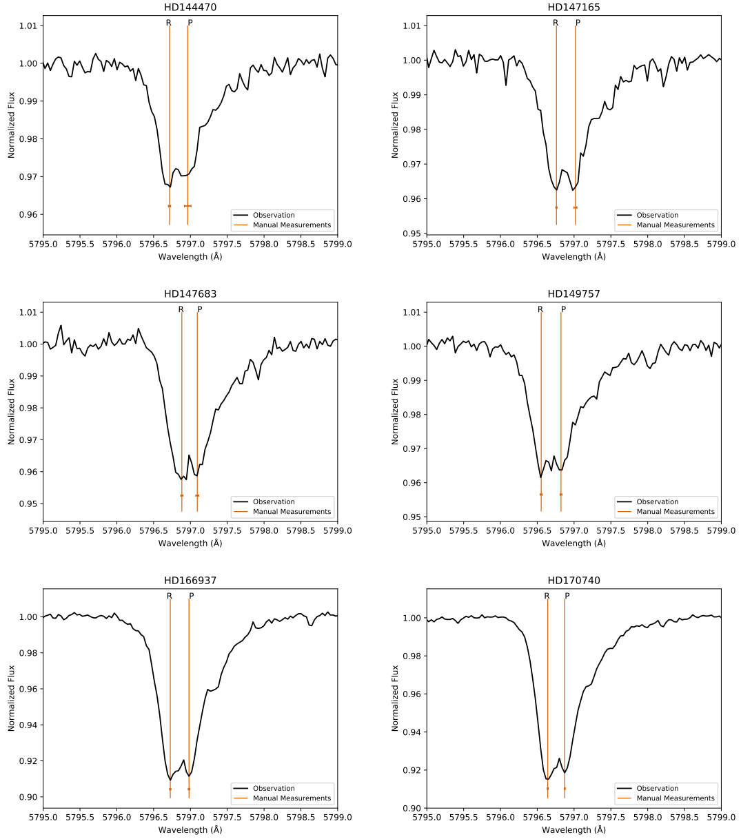
Fig. D.1. Same as Fig. C.1 but for the 5797 Å DIB.
