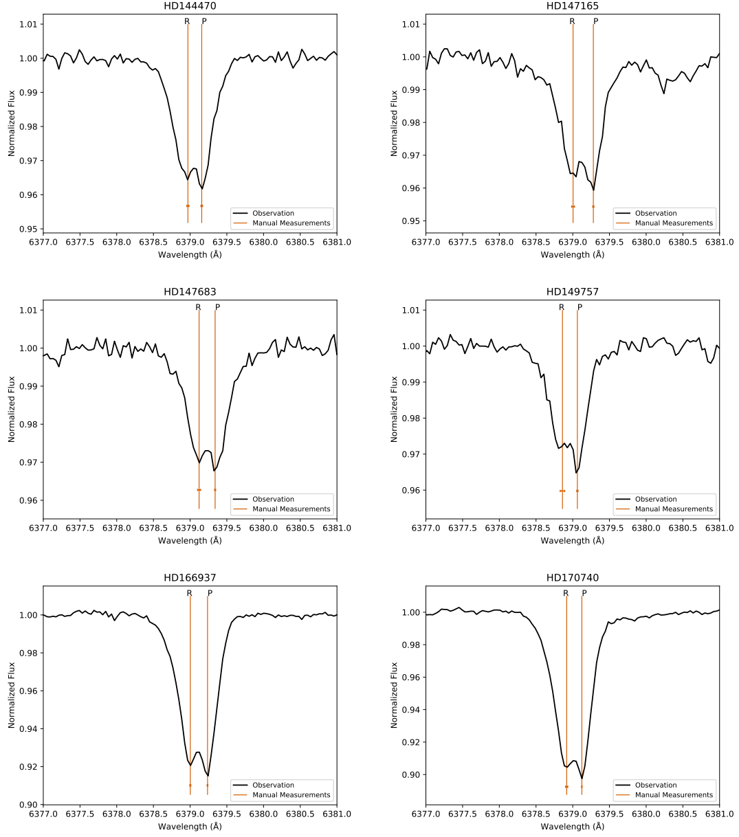
Fig. E.1. Same as Fig. C.1 but for the 6379 Å DIB.
