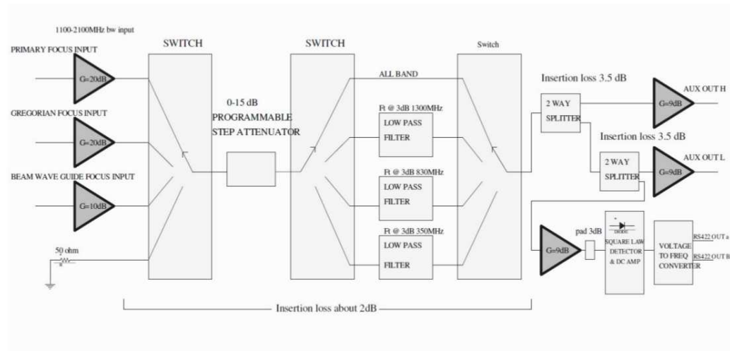
Fig. 1. Focus Selector.
