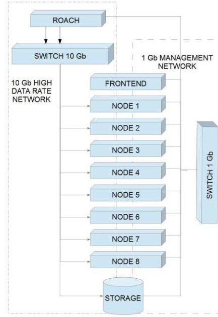
Fig. 9. ROACH/cluster/storage system, composed by a Roach board and 8 CPU based computing nodes
