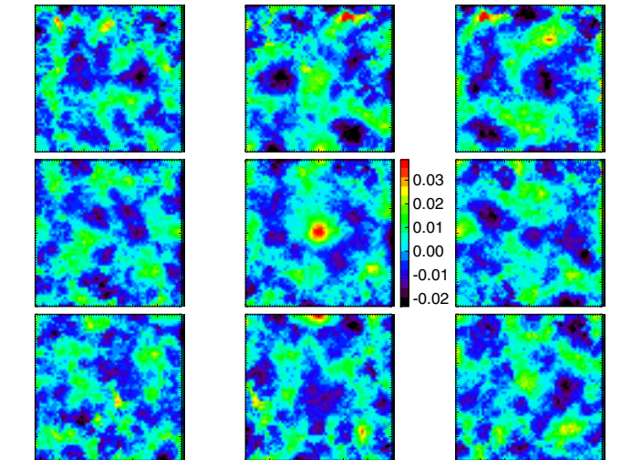
Fig. 3. Tests of stacking on “depainted” regions. The central panel shows the stacked result obtained at 857 GHz for the 645 cluster-centred patches (as in Fig. 2). This is surrounded by the eight neighboring maps obtained by changing the cluster Galactic longitude or latitude (or both) by \pm 1^\circ .
