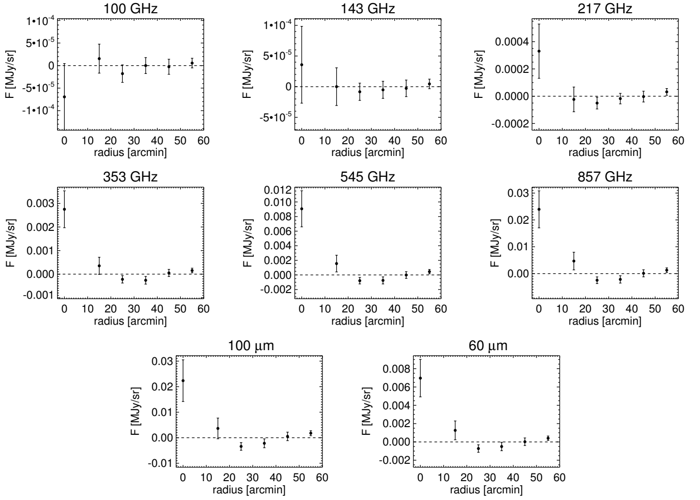
Fig. A.1. Radial profiles obtained from the background- and foreground-cleaned stacked maps, for the sample of 645 clusters. The units here are MJy sr -1 . The black points correspond to the values obtained as the average of the pixels contained within each region considered and associated uncertainties have been obtained using bootstrap resampling. We find no significant detection at 100 and 143 GHz, while the detection starts to become strong at \nu \geq 353 GHz, consistent with what we saw in Fig. 2.
