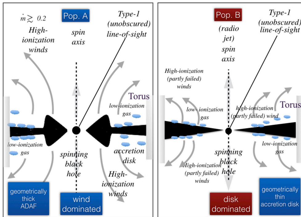
FIGURE 6 | Different structure for Pop. A (left) and B (right), with a slim and a flat disk respectively. The sketch is not drawn to scale and the relation between line emitting regions (shown here as clouds) and accretion disk structure is still debated. See section 8.1 for a more detailed explanation.
