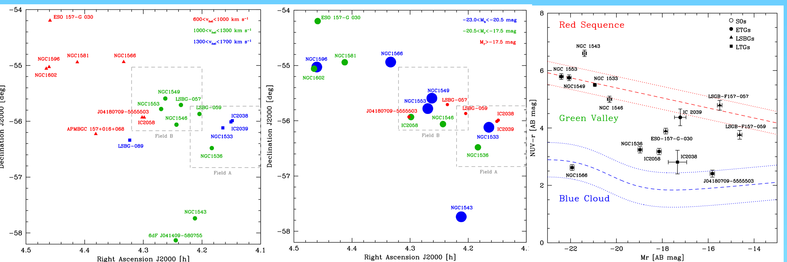
FIG.1 (top panels) The Dorado group partially covered by two VST fields. (bottom left panel) The observed fields are indicated by grey dashed lines. Member galaxies according to Firth+ (2006) are separated in velocity bins: the dynamical analysis suggests that Dorado is not yet virialized: galaxy clumps are still present. (mid bottom panel) Giant members are divided in bins of absolute magnitude M r , adopting the distance D=16.9 Mpc : the group backbone marked by giants is shown in blue, dwarfs in red. (right bottom panel) The (NUV-r) vs M r color magnitude diagram. The RS and the BC in Dorado, represented by dashed lines, are averages from Wyder+ (2007). Member galaxies are divided by morphology (full circle=Es, open circle= Spirals, low surface brightness galaxies=triangles).
