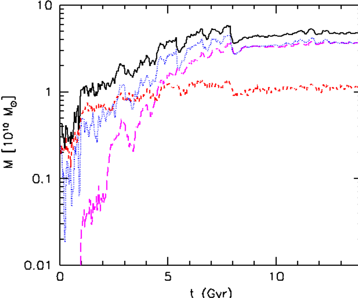
FIG.3: (top) the global observed SED of NGC 1543 (dots) and that predicted (solid red line) by a minor merger (5:1) of total initial mass 2.4x10 11 M ⊙ at the age of 10.6 Gyr. (middle) The predicted evolution in the rest-frame (galaxy frame) CMD (red triangles correspond to z=1, 0.5 and 0, respectively). (bottom) The mass assembly, computed inside, R 25 : (magenta) stars, (red) dark matter, (blue) gas, and (black) the total mass (Mazzei et al. 2018 in prep.).
