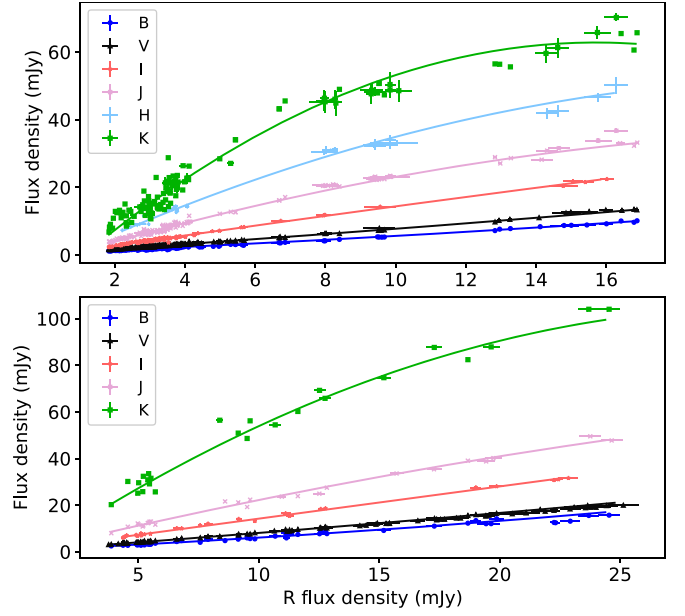
Figure 5. BVJHK vs. R -band flux densities for the 2013 (upper panel) and 2014 flares (lower panel).
