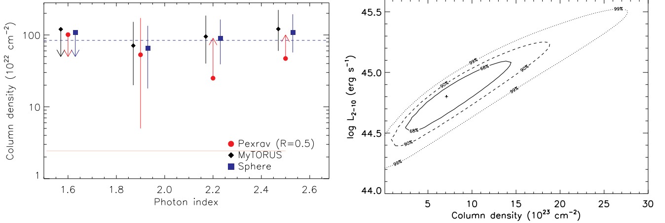
Figure 7. Left panel: Values of the column density N_{\text{H}} obtained by assuming different values of the photon index of the primary X-ray radiation for the PEXRAV, MYTORUS and SPHERE models. The points obtained with the last two models have been shifted by \Delta\Gamma = \mp 0.03 for visual clarity. The dashed line shows the value of N_{\text{H}} obtained from E(B - V) by using Eq. 1 (see also Table 3). Right panel: Confidence intervals of the intrinsic 2–10 keV luminosity and the column density for WISE J1036+0449 obtained using the MYTORUS model. The continuous, dashed and dotted lines represent the 68%, 90% and 99% confidence contours, respectively. The black cross represents the best-fit value of the parameters.
