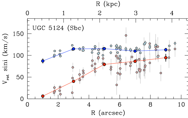
FIG. 16.— Detection of asymmetric drift in the MaNGA prototype observations of UGC 5124 (p9-61A), which has an inclination of i = 45^\circ 6 \pm 2^\circ 0 and a distance of 87.8 Mpc. Small, light-blue and light-red points are measurements of ionized-gas and stellar velocities, respectively, as a function of disk-plane radius ( R ) from individual fibers that have been projected onto the major axis of rotation. Only those data within \pm 60^\circ (disk-plane azimuth) of the major axis have been plotted. Large blue and red points show the error-weighted mean, projected rotation speed ( V_{\text{rot}} \sin i ) in 2'' bins for the ionized-gas and stellar components, respectively. As expected, the stellar (red) component lags behind the ionized-gas (blue) component owing to the substantially larger velocity dispersion and collisionless nature of the stars.
