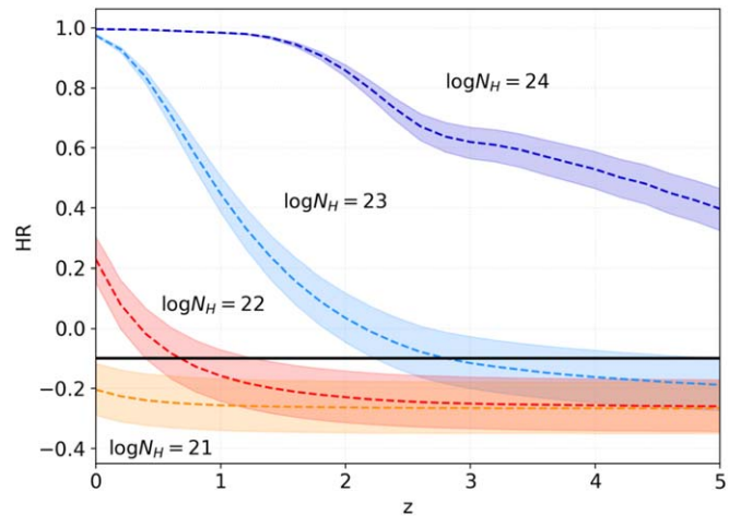
Figure 2. The HR as a function of redshift for different absorption column densities in color code. The shaded areas indicate HR values derived with fixed \Gamma = 1.7 (top curves) and \Gamma = 2.1 (bottom curves), while the dotted lines represent models with \Gamma = 1.9 . We used the response matrices at the aimpoint of the Chandra observations. The black horizontal line represents the chosen selection threshold \text{HR} = -0.1 .
