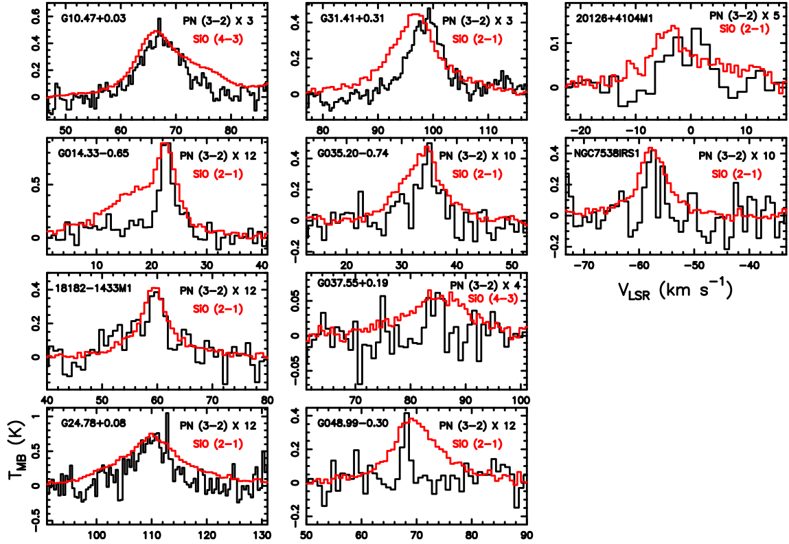
Figure 8. Comparison between the profiles of the PN (3–2) line (black) and the SiO (2–1) or (4–3) lines (in red). The x-axis represents a velocity interval of (-20, +20) km s ^{-1} centred on the LSR velocity of each source, as in Fig. 2.
