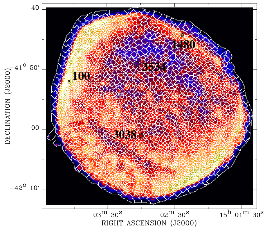
Figure 2. Tessellated meshes used for spatially resolved spectroscopy analysis (the high-resolution run) overlaid on the 0.3–8 keV image of SN1006. There are in total 3596 regions, each containing \geq 10^4 counts from the combination of MOS-1, MOS-2, and PN. The four black meshes are the regions used to extract the sample spectra in Fig. 3, with the region numbers denoted beside.
