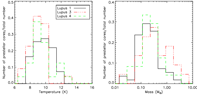
Fig. 10. Normalised distribution of the temperature (left panel) and mass (right panel) of the population of prestellar cores in the three Lupus clouds. On the y -axis, the number of objects per bin relative to the total number of prestellar cores in each cloud is reported.
