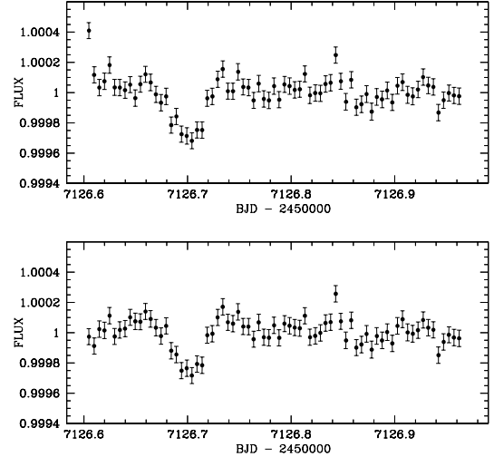
Fig. 10. Spitzer photometry divided by two different best-fit baseline models. The first (top) aims to remove position- and PSF effects, and consists of a 4th order polynomial of the PSF x - and y -centres and widths, supplemented with the BLISS mapping method (Stevenson et al. 2012) to remove high-frequency position effects. The second baseline model (bottom) adds to the first a slope and a quadratic function of the logarithm of time to model the sharp decrease in the counts at the beginning of the run (negative ramp). Both light curves are binned per 0.005d = 7.2 min intervals.
