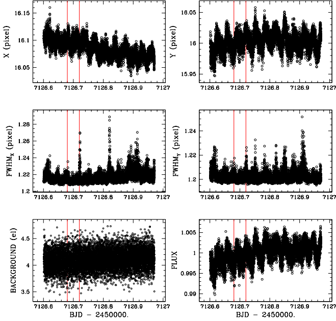
Fig. 9. Evolution of the following measured parameters in the Spitzer images for HD 219134: PSF centre x - and y -positions (top), PSF x - and y -widths (middle), background counts (bottom left), and stellar fluxes (bottom right). The times of the start and end of the detected transit are shown as red vertical lines.
