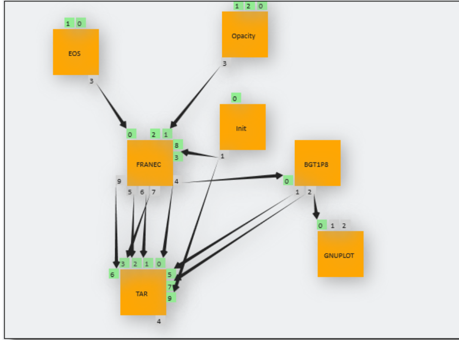
Figure 3: FRANEC workflow.
