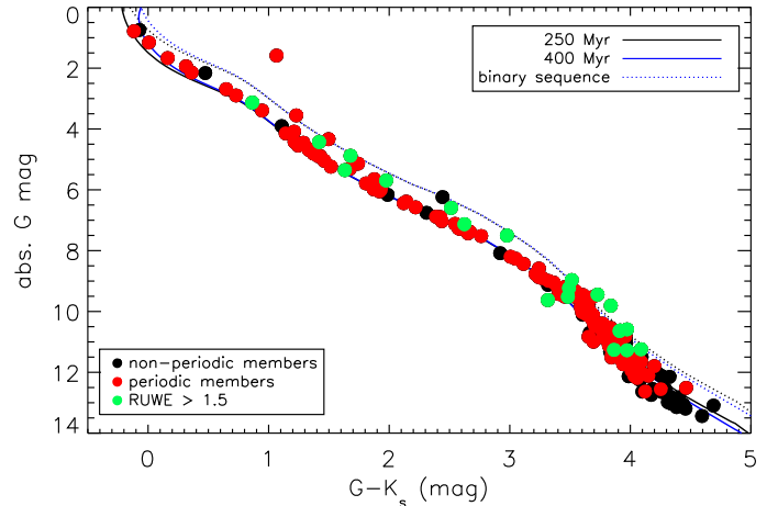
Fig. 1. CMD for the Group X candidate members ( Tang et al. 2019 ), with the 250 Myr (solid black line) and 400 Myr (solid blue line) isochrones overplotted. Dashed lines represent the sequence of equal-mass main-sequence binaries. Errors on magnitudes and colours are smaller than the symbol size.
