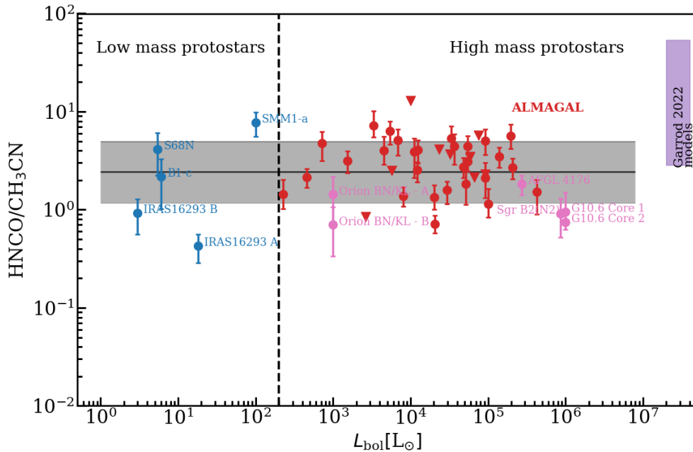
Fig. 10. Same as Fig. 9, but for HNCO/CH_3CN . The literature values are taken from studies presented in Table E.4. In this plot SMM1-a is colored blue although it is an intermediate mass protostar.
