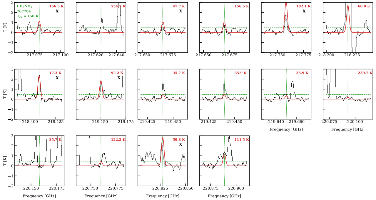
Fig. D.5: Showing that excitation temperature of 150 K does not match the observations for \text{CH}_3\text{NH}_2 in source 767784. The various symbols are the same as Fig. 2. Again here some lines are overestimated and if the column density is decreased the lines that are perfect fits now will be underestimated.
