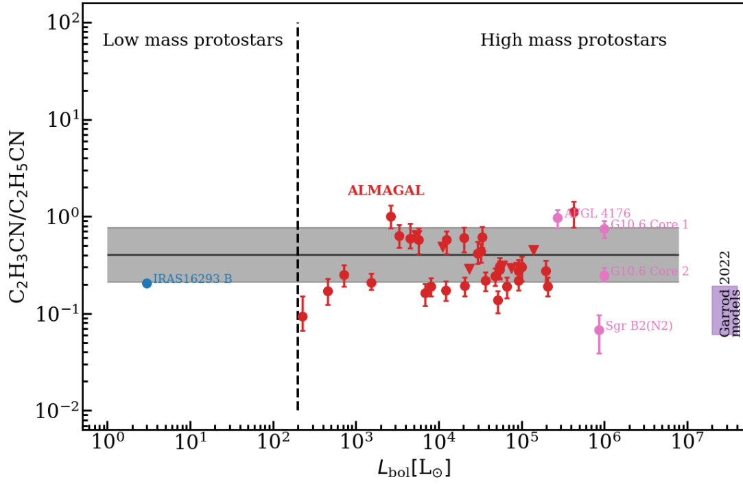
Fig. D.19: Same as Fig. 9, but for \text{C}_2\text{H}_3\text{CN}/\text{C}_2\text{H}_5\text{CN} . The references are given in Table E.4.
