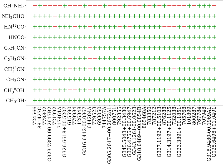
Fig. D.16: Same as Fig. 4, but now the sources are ordered from left to right from the lowest to highest luminosity.
