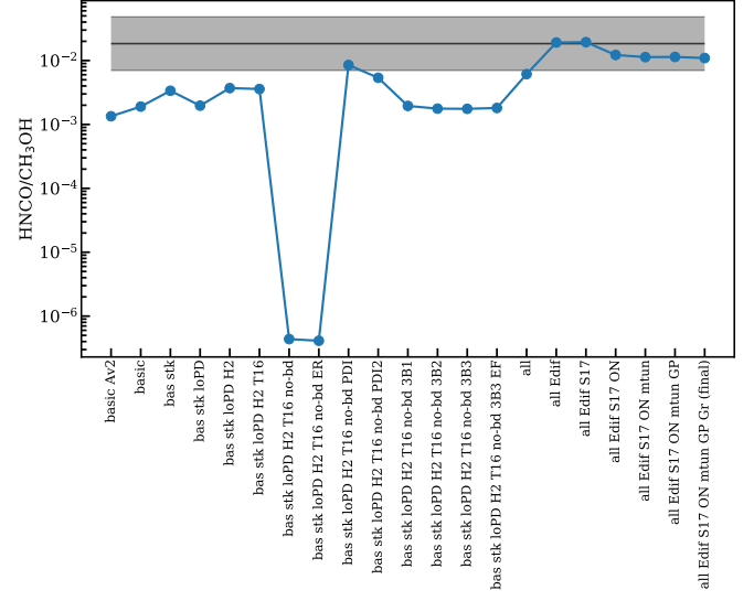
Fig. D.31: Same as Fig. D.29, but for \text{HNCO}/\text{CH}_3\text{OH} .
