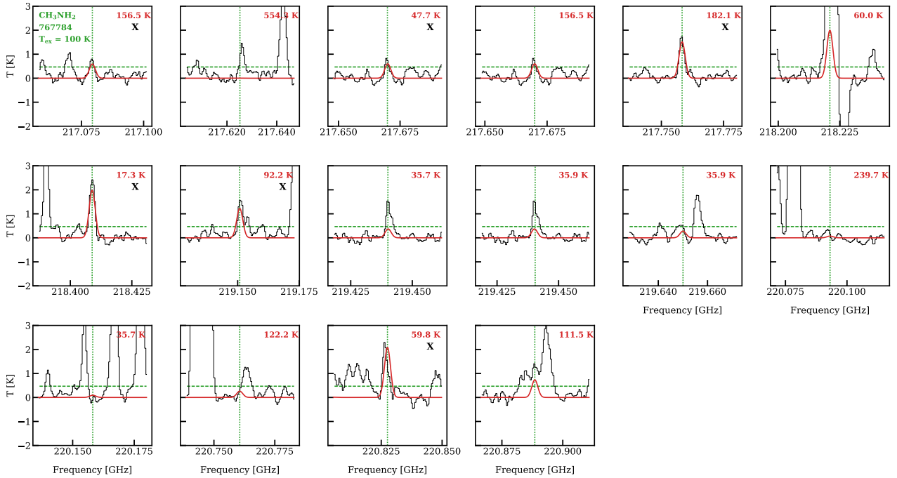
Fig. D.4: Best-fit model for \text{CH}_3\text{NH}_2 in source 767784. The various symbols are the same as Fig. 2.
