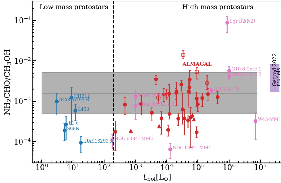
Fig. 11. Same as Fig. 9, but for \text{NH}_2\text{CHO}/\text{CH}_3\text{OH} . The red hollow circles indicate the sources for which ^{13}\text{CH}_3\text{OH} was used to find the column density of \text{CH}_3\text{OH} .
