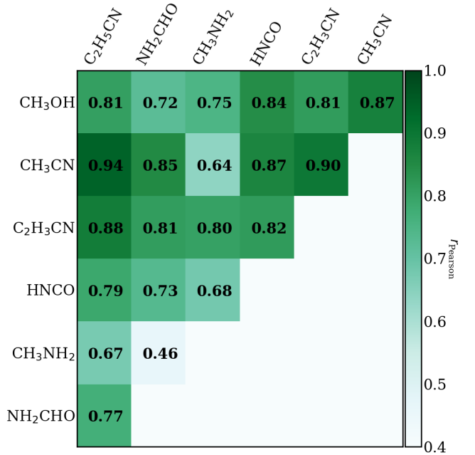
Fig. 7. Correlation matrix for Pearson coefficient of the column densities. The darkest green shows the highest correlation. In this figure sources with their methanol column density found from ^{13}\text{CH}_3\text{OH} are excluded due to optical depth effects.
