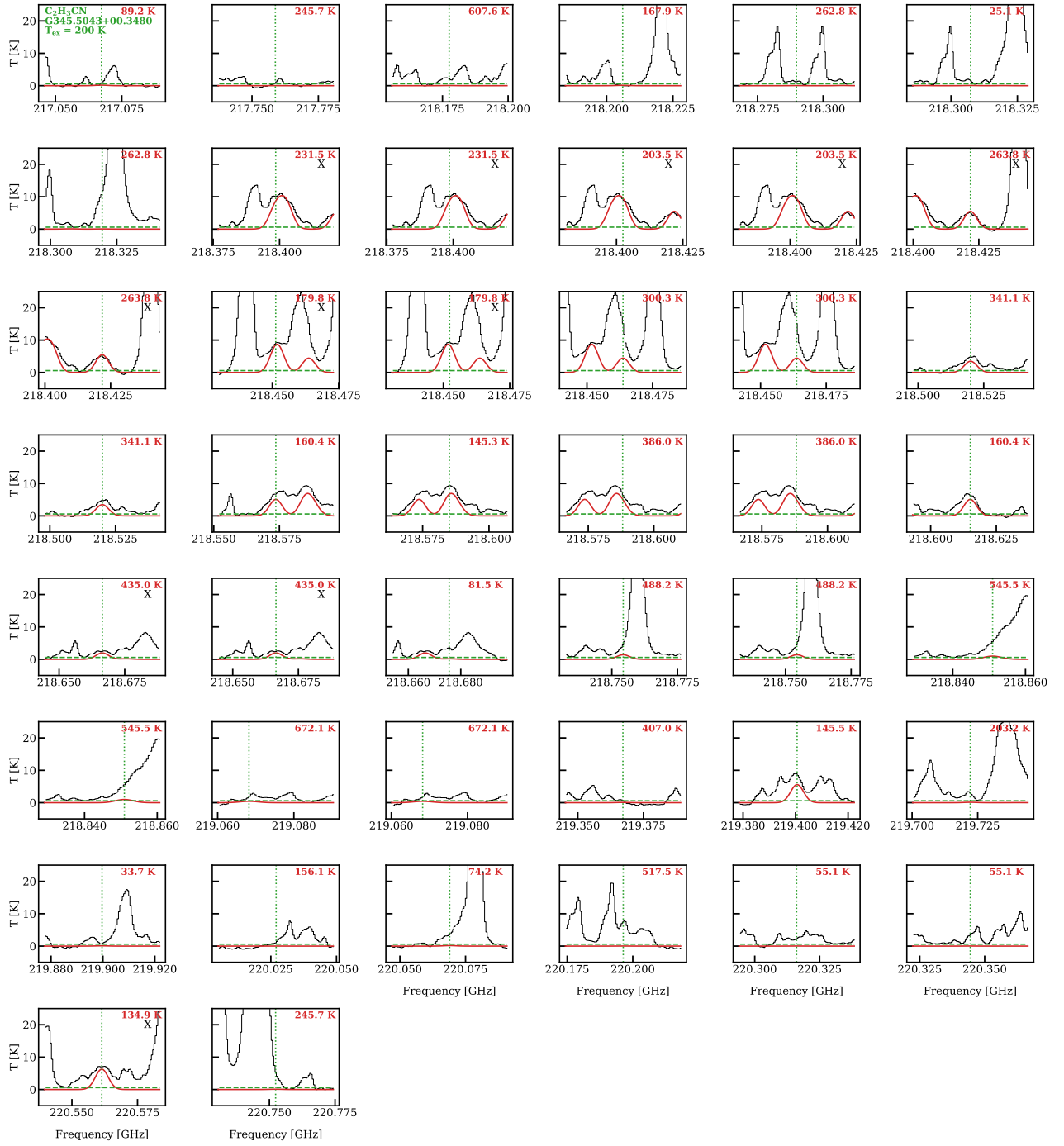
Fig. D.11: Same as Fig. D.6, but for G345.5043+00.3480 and C_2H_3CN .
