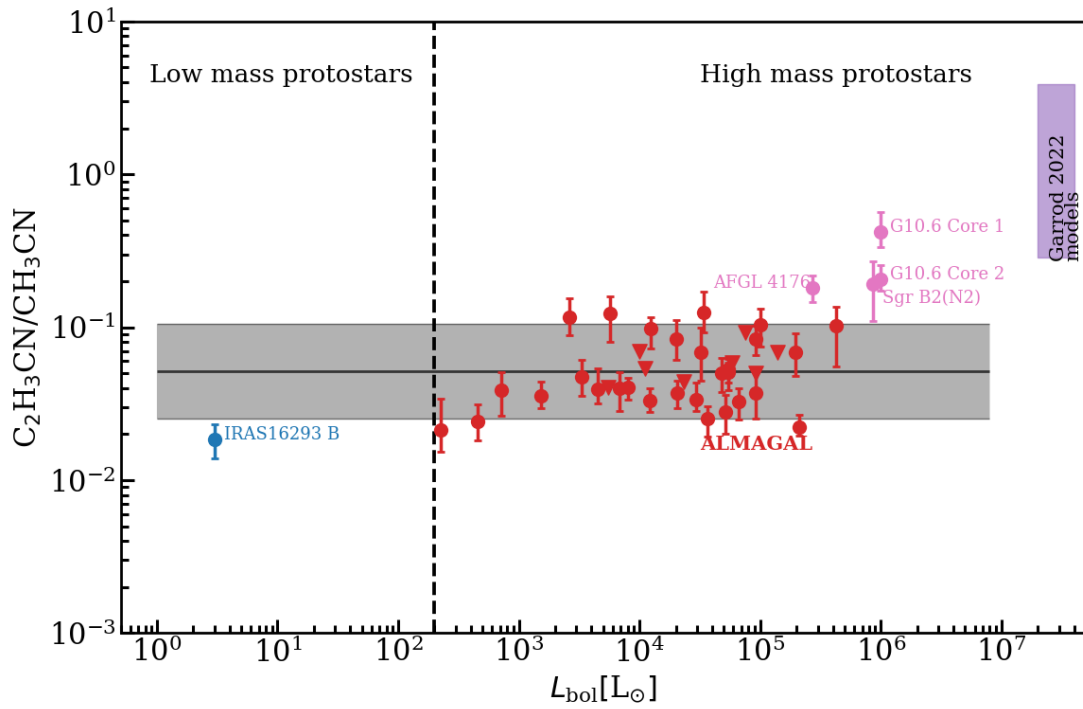
Fig. D.20: Same as Fig. 9, but for \text{C}_2\text{H}_3\text{CN}/\text{CH}_3\text{CN} . The references are given in Table E.4.
