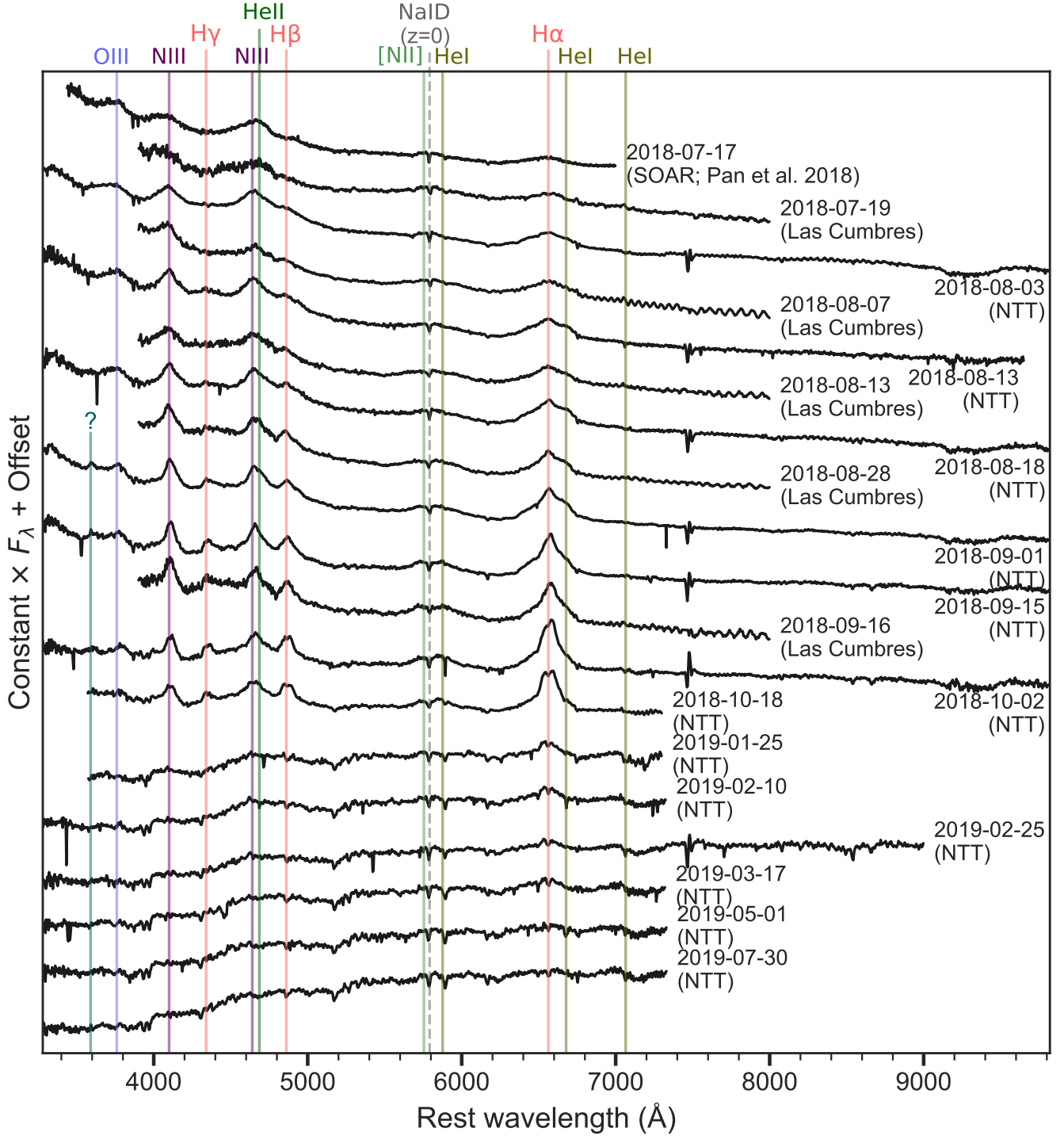
Figure 2. The low-resolution spectra of AT 2018dyb with the strongest broad lines identified. The SOAR spectrum (Pan et al. 2018) has been retrieved from the TNS.
