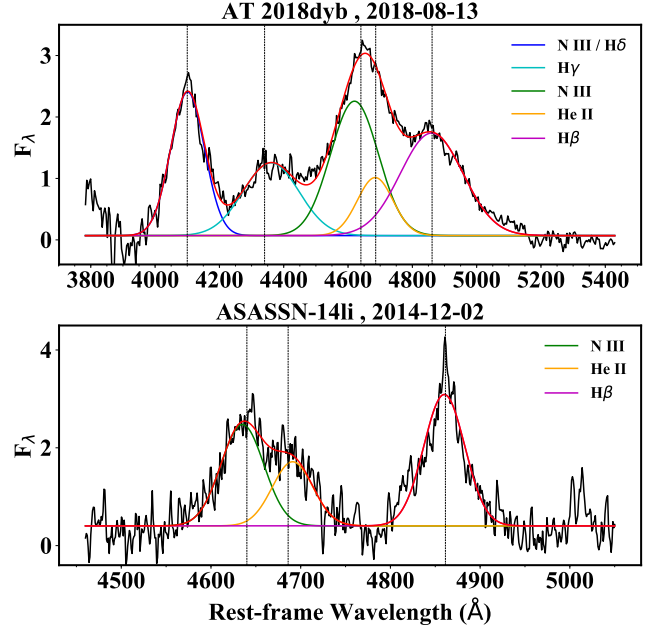
Figure 5. Upper panel: example of a simultaneous fit with five Gaussians in the spectrum of AT 2018dyb. The central wavelengths of the lines at zero velocity have been marked with dashed lines. Lower panel: similar but for ASASSN-14li. For this TDE the lines are narrower and do not blend as severely as for AT 2018dyb. For this reason, it not necessary to fit five lines simultaneously. Here, we show a triple fit focusing on N III, He II and H \beta .
