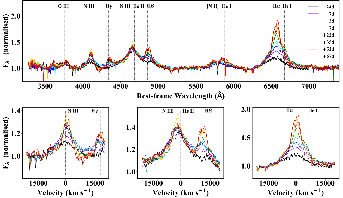
Figure 3. Upper panel: selected spectra of AT 2018dyb after normalising with the continuum, overplotted with different colors as indicated in the legend. The phases refer to the time of U -band maximum and they are given in the rest frame. The strongest lines have been identified. All lines grow stronger with time and this is particularly true for the Balmer lines. Lower panels: a zoom-in on some of the strongest lines in velocity space. In the middle panel, the zero velocity has been set considering He II, but it can be seen that the line peaks between He II and N III and that it is likely a blend. The width of the lines starts at \sim 12,000 km s ^{-1} and decreases with time (see also Figure 6).
