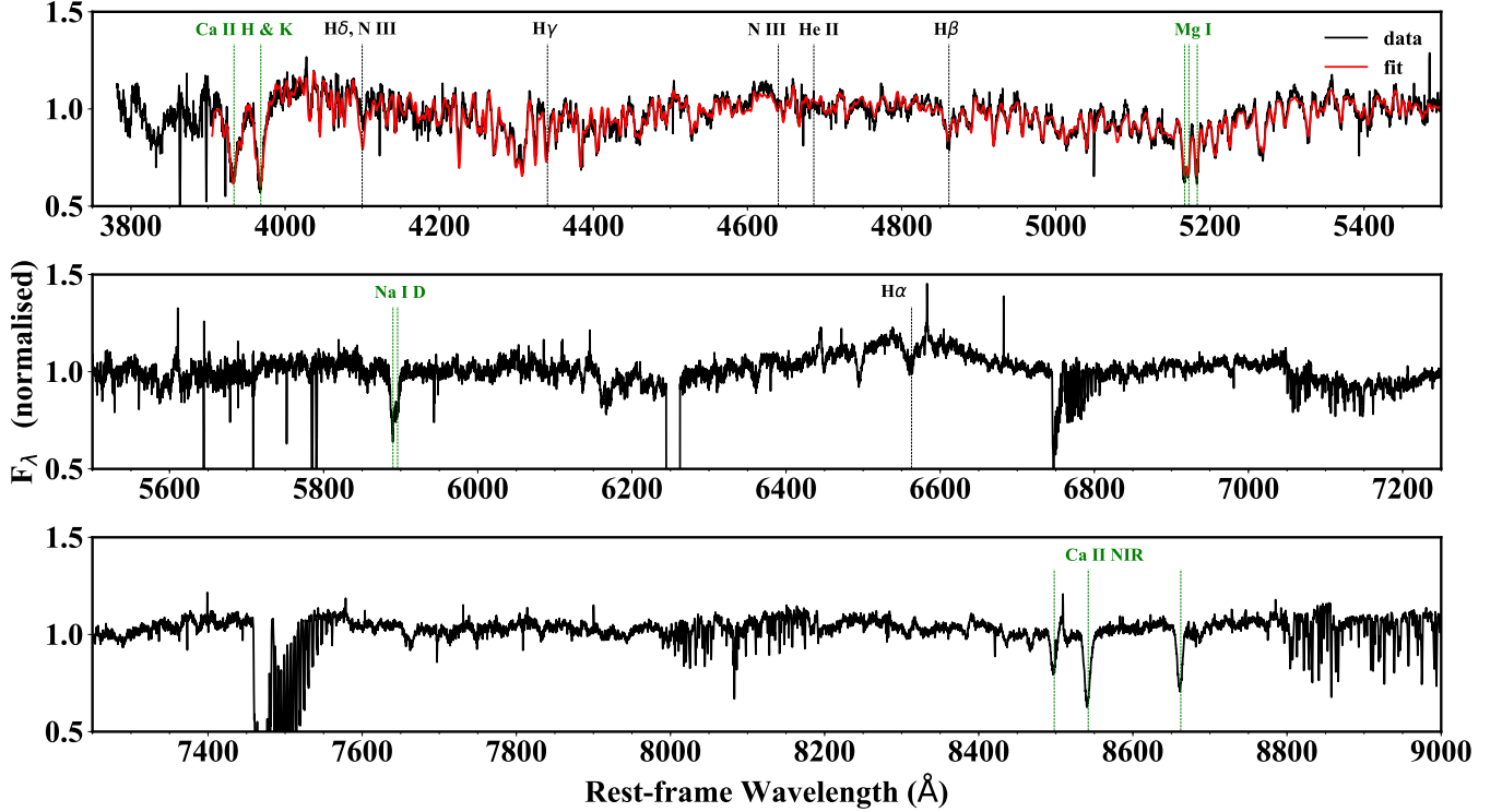
Figure 9. The X-shooter spectrum of AT 2018dyb obtained 206 days after maximum light (normalised). The UV part has been fit by PPXF to determine the velocity dispersion at the host. The same lines have been marked as in previous figures for comparison: broad lines with black and narrow absorption lines with green dashed lines. With the exception of H\alpha , the broad lines that were prominent at early phases have disappeared.
