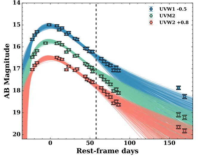
Figure 11. Best-fit light curves from MOSFiT. The fit only uses UV observations out to the dashed line at rest-frame day +58.2 (MJD = 58400). As shown in Section 7, host contamination is negligible for these data and all the light comes from the TDE. The light curves have been extrapolated out to later times for the plot.
