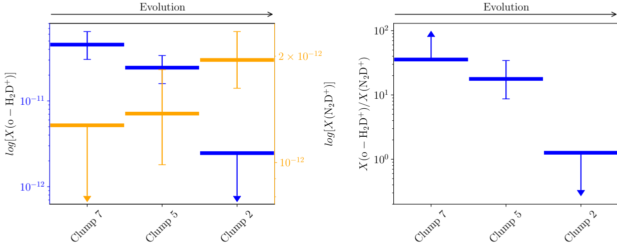
Fig. 3. Left: Calculated o-H 2 D + (blue) and N 2 D + (orange) abundances. Right: Relative abundance of the two species. The clumps are ordered by evolutionary stage, from the least- to the most evolved. The 95% credible interval is indicated for abundances and ratios; we point out that for non-detections, only the upper limit is shown.
