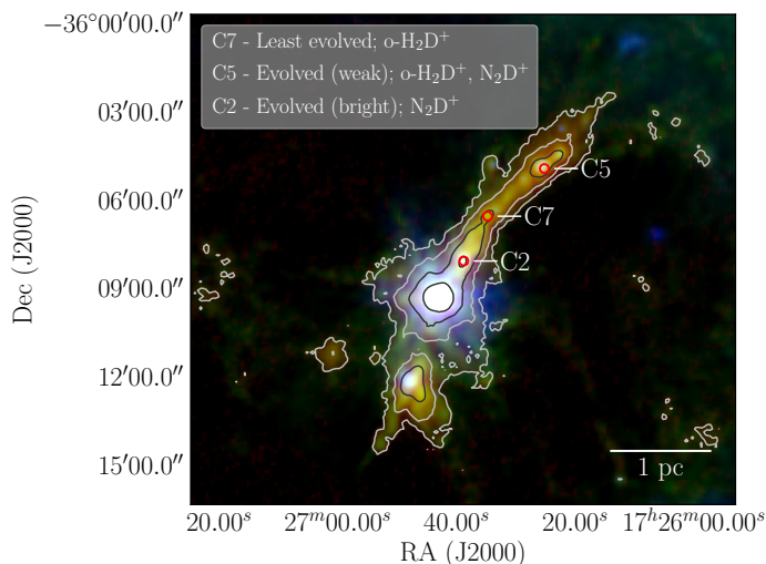
Fig. 1. Three-colour image (red: ATLASGAL 870 \mu\text{m} , green: Hi-GAL 250 \mu\text{m} , blue: Hi-GAL 70 \mu\text{m} ) of the G351 complex. Contours of the ATLASGAL images are also indicated in grey (0.15, 0.5, 1.5, 5 \text{Jy beam}^{-1} ). Clumps 2, 5, and 7 are indicated in red. In the top-left corner we list the clumps from the least- to the most evolved, and the species we observed in each source.
