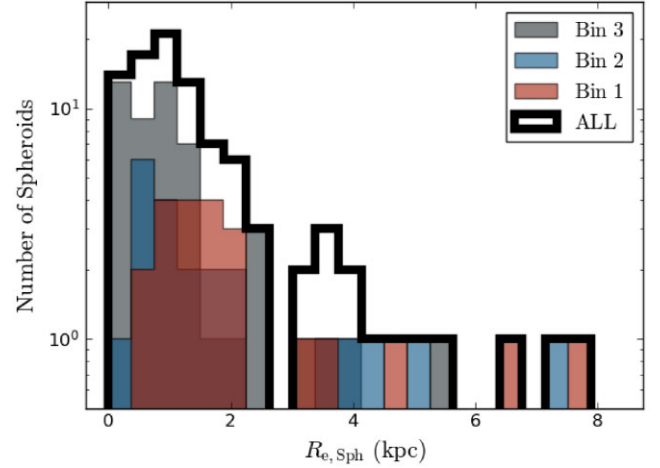
Figure 11. The size ( R_{e, \text{Sph}} , in equivalent axis) distribution of our bulges/spheroids. The spheroids from Bins 1, 2, and 3 are depicted by the red, blue, and black histograms, respectively. The thick black line depicts the size distribution of the entire sample set. The figure only shows the 96 spheroids with R_{e, \text{Sph}} < 10 kpc of the complete sample, see the spheroids’ size–mass distribution later in Section 4.3 for further reference.
