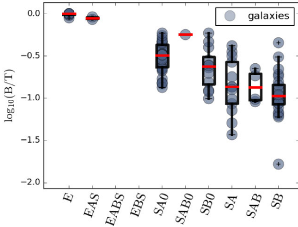
Figure 12. SDSS i -band Bulge-to-Total ( B/T ) flux ratios. The spiral (SA–SB) galaxies presented here are dominated by the so-called ‘early-type’ spirals (Sa–Sb). The boxes denote the lower (Q1) to upper (Q3) quartiles of the data, and the whiskers extend from the minimum to the maximum data points (excluding any outliers). The red lines represent the median \langle B/T \rangle ratios for each morphology. The ‘+’ marker denotes an outlier (NGC 5350) that lies beyond the Q1 - 1.5(Q3 - Q1) limit (Tukey 1977).
