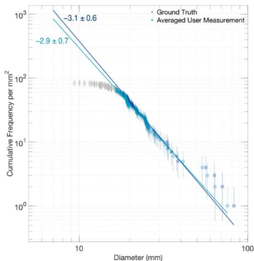
Figure 5. Cumulative PSFDs of caliper measurements and remotely sensed measurements. Light gray points indicate particle measurements that were smaller than the completeness limit. Error bars represent Poisson detection distribution uncertainty (square root of N_C ).
