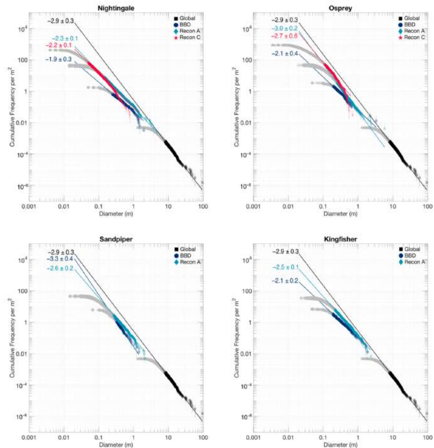
Figure 6. Cumulative PSFDs of Bennu for the four candidate sample sites as calculated at several key mission phases. Recon C mapping was only performed for the primary and back-up sample sites, Nightingale and Osprey. The global PSFD calculated from early OSIRIS-REx images of Bennu by DellaGiustina and Emery et al. [24] is included as a reference. Light gray points indicate particle measurements that were smaller than the completeness limit.
