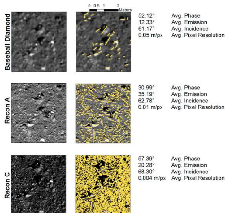
Figure 1. Close-up examples of images of Bennu's surface with and without mapped particles. This example falls within the Nightingale region. Illumination conditions and pixel resolution are included for context. We define incidence as the angle between the light vector and the surface normal (Sun-Bennu-surface normal), emission as the angle between the observation vector and the surface normal (OCAMS-Bennu-surface normal), and phase as the angle between the light vector and observation vector (Sun-Bennu-OCAMS).
