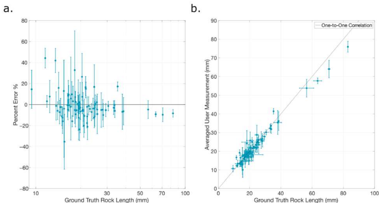
Figure 4. (a). Percent error between remotely sensed and ground-truth measurements. (b). Correlation plot between caliper measurements and remotely sensed measurements. Both panels demonstrate the slight trend of overestimating the measurement of small particles and underestimating the measurement of large particles. Vertical error bars represent the uncertainty in the remote measurements amongst all of the counters. Horizontal error bars represent the uncertainty in the caliper measurements.
