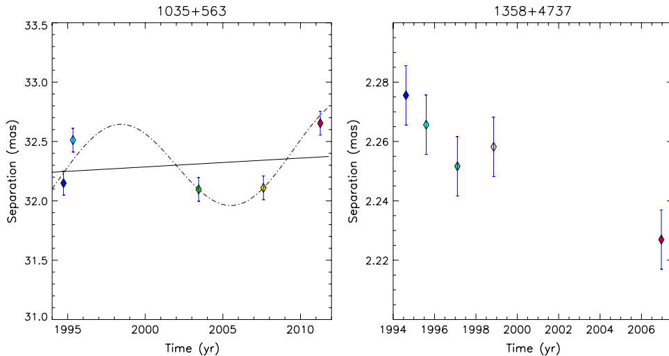
Figure 1. Left panel Separation versus time in J1035+5628. Data are taken in X-band. Right panel Separation versus time in J1358+4737. Data are taken in C-band
