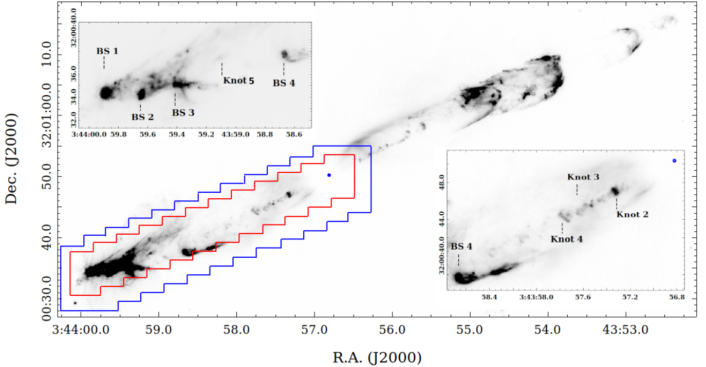
Fig. 1. MIRI-MRS map coverage of the HH 211 outflow (Channel 1 in red and Channel 4 in blue). The F460M NIRCcam image at 4.6\ \mu\text{m} in grey scale is from Ray et al. (2023). The blue circle marks the HH 211 mm position as observed with ALMA by Lee et al. (2019). The zoomed-in inset in the top left corner shows the blueshifted terminal BSs and the inset in the bottom right corner shows the main knots along the blueshifted jet.
