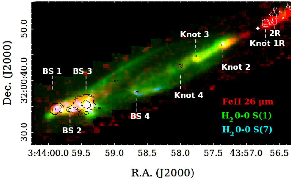
Fig. 3. Tricolour MIRI-MRS map of \text{H}_2 0-0 S(7) (at 5.5\ \mu\text{m} , in blue), \text{H}_2 0-0 S(1) (at 17\ \mu\text{m} , in green), and [Fe II] (at 26\ \mu\text{m} , in red) emission lines. The white circle marks the position of the ALMA mm continuum source. Black and white contours indicate the position (on the blue- and redshifted lobe side, respectively) of continuum emission integrated between 25.3 and 25.9\ \mu\text{m} (displayed contours are at 3 , 5 , and 50\sigma ; 1\sigma=4\ \text{MJy sr}^{-1} ). Knots and bow shocks showing continuum emission are indicated.
