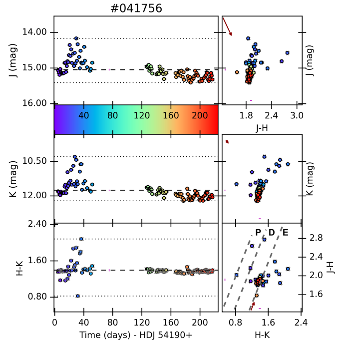
Fig. 11. Disk-bearing (Class II) star CygOB2-041756 ( S = 10.4 ) is an example of a mixed variable with a long term variability mixed with burst features in the first epochs observed. The star is a compound variable with asymmetries in the light curve having a distinct color behavior. The plots, colors, and symbols are the same as in Fig. 4.
