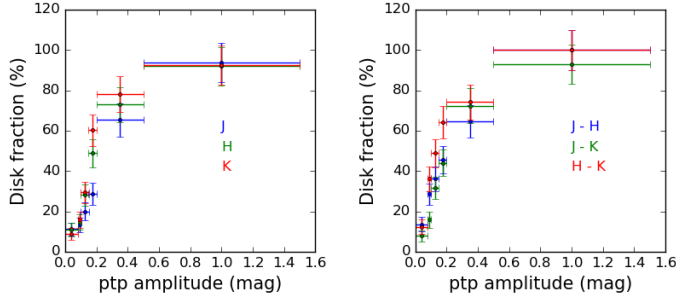
Fig. 3. Disk fraction as a function of peak to peak amplitude for each near-IR band ( left ) and color ( right ). In both plots, circles show the center of each ptp amplitude bin and horizontal bars indicate the size of each bin. Vertical bars show the standard errors of a Poisson counting in that bin.
