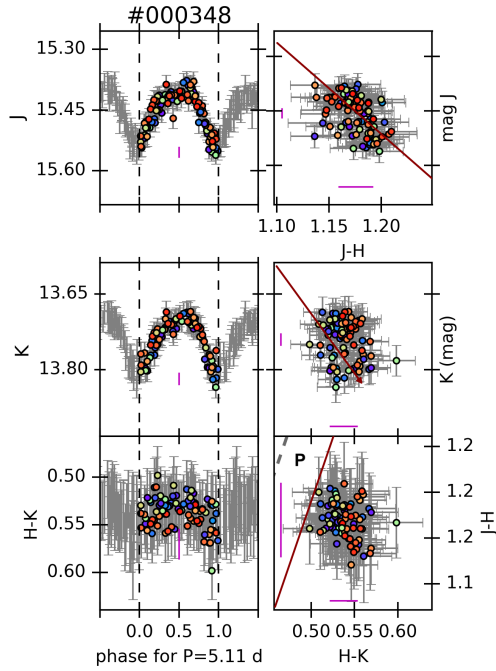
Fig. 5. Star CygOB2-000348 is an example of a diskless periodic variable, with S = 1.62 , a ptp amplitude of 0.13 and 0.11 mag in the J and K bands respectively, and that does not show periodicity in color. The plots, colors, and symbols are the same as in Fig. 4, but with the light curves and color curve phased with the period of the star, P = 5.1 d.
