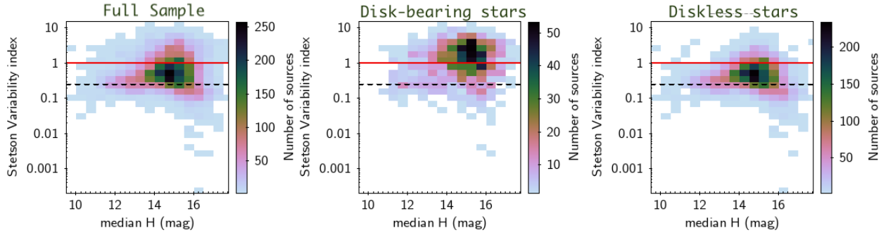
Fig. 2. Distribution of Stetson variability index as a function of H median magnitude for the full sample of candidate members ( left ), disk-bearing stars ( middle ), and diskless stars ( right ). The red line shows S = 1 , and the dashed black line shows S = 0.25 .
