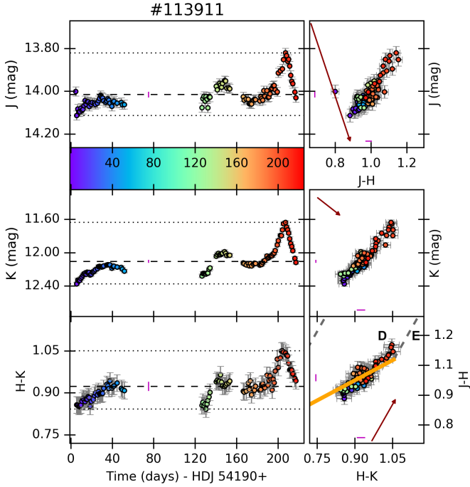
Fig. 9. Disk-bearing (flat-spectrum) star CygOB2-113911 is an example of a long-term variable with S = 3.67 , that presents a blueing linear trajectory in the color-magnitude diagrams. The plots, colors, and symbols are the same as in Fig. 4.
