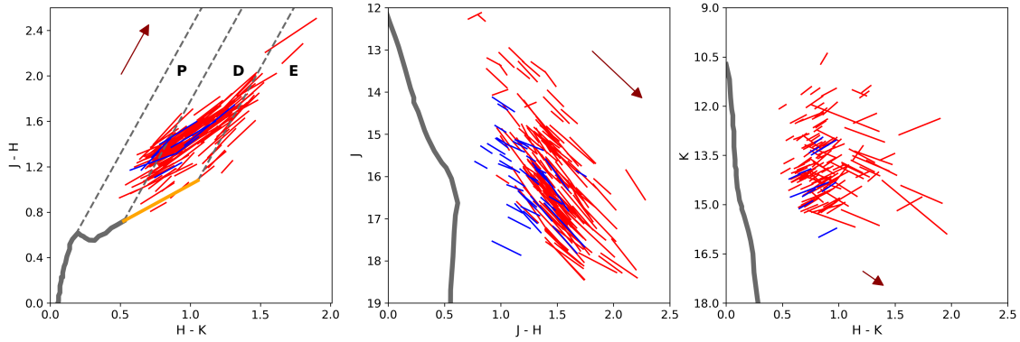
Fig. 10. Color-magnitude and color-color diagrams with the slopes for the stars presenting a linear variation. Red lines show disk-bearing stars, and blue lines show stars without discs. The length of each line segment reflects the amplitude of the variability. The dark red arrows show the median interstellar extinction toward CygOB2, and the gray lines show as reference of unreddened normal photosphere colors, an empiric isochrone from Kraus & Hillenbrand (2007).
