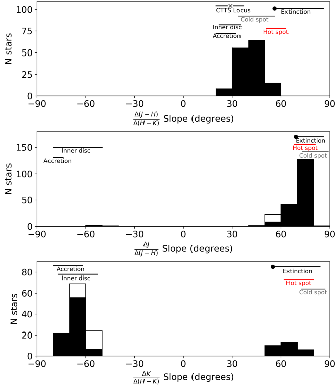
Fig. 14. Distribution of slopes measured in the color-color and color-magnitude diagrams. The figure shows slopes for J-H vs. H-K (top), J vs. J-H (middle), and K vs. H-K (bottom) diagrams. We plotted the expected slopes for each physical mechanism as line segments, following the ranges in Table 7. The X mark shows the exact position of the T Tauri Locus. The black circle shows the slope expected for the typical dust opacity index in the ISM. Black bars show the stars in S_1 sample and with precision in the light curve better than 5%, empty bars show stars in the S_2 sample or with precision worse than 5%.
