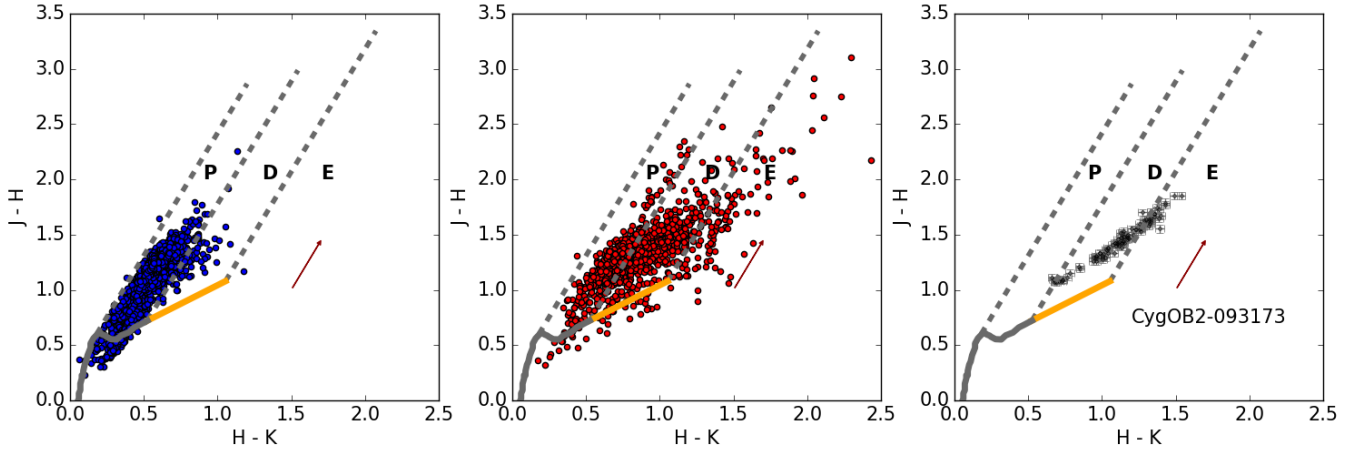
Fig. 1. Near-IR ( JHK ) color-color diagrams. Left and middle panels: median colors of the 3811 diskless stars (blue dots) and the 1272 disk-bearing stars (red dots) analyzed in the present study. Right panel: CygOB2-093173 variable star. Black dots show the color of the star in each observed night. The regions labeled as “P”, “D”, and “E” are the regions typically occupied by stars with normal photospheric colors, disk-bearing colors, and extreme near-IR excess respectively. The dark red arrow shows the effect of the interstellar reddening for the median visual extinction expected for stars in the CygOB2 association ( A_V = 4.1^m ). The gray solid curve shows an empirical dwarf sequence by Kraus & Hillenbrand (2007) and the orange line shows the Meyer et al. (1997) T Tauri locus. Dashed gray lines show extinction paths of A_V = 10^m for 0.6 M_\odot and 0.08 M_\odot stars, and the truncation point of the T Tauri locus.
