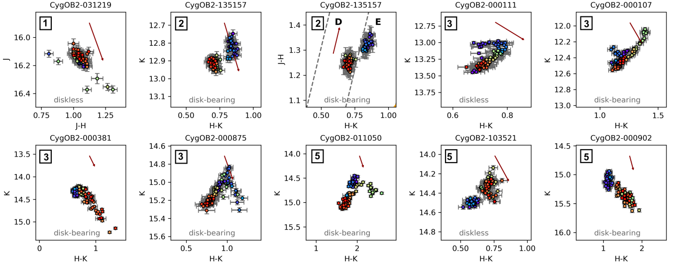
Fig. 13. Examples of stars with a compound behavior are shown inside color-color diagrams or color-magnitude diagrams. 1- Asymmetry with a distinct color; 2- Variable IR-excess; 3- Changing slope; 5- Mix of 2 and 3. Dark red arrows show the effect of interstellar reddening for A_V = 1 mag. The color of each data point reflects its observational date following the color-bar in Fig. 4.
