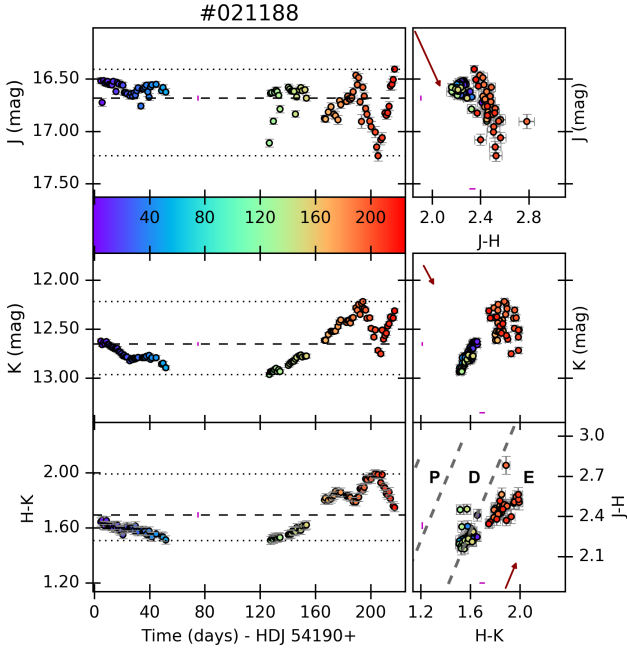
Fig. 12. Disk-bearing (Class II) star CygOB2-021188 ( S = 1.0 ) is an example of compound variability showing a variable near-IR excess and a changing slope during the observed time. The plots, colors, and symbols are the same as in Fig. 4.
