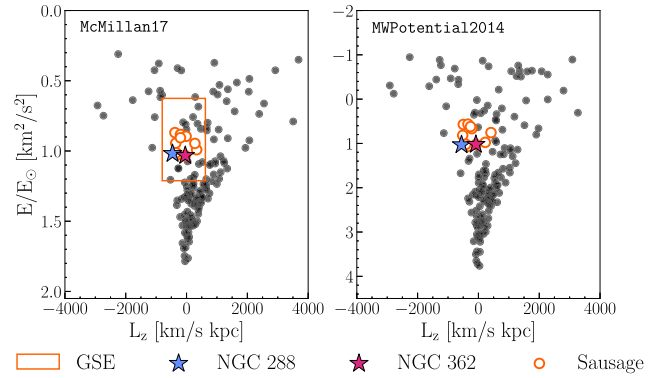
Figure 1. Energy ( E in \text{km}^2/\text{s}^2 ) scaled by solar energy versus angular momentum ( L_z in \text{km/s kpc} ) for the majority of MW GCs calculated using the McMillan17 MW potential (as in the studies of Myeong et al. 2018; Massari et al. 2019), integrating for 2 Gyr (left). The extent of GSE in E versus L_z as defined by Massari et al. (2019) is marked in orange, while the Sausage GCs identified by Myeong et al. (2018) are shown as the open orange circles. NGC 288 and NGC 362 are shown as the blue and pink stars, respectively. The same information is shown for GCs integrated in the MWPotential2014 MW potential (right).
