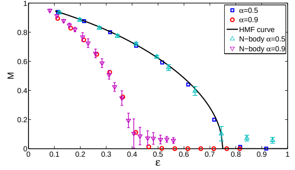
Fig. 4: Comparison between the analytic magnetization curves and the data recorded via N -body simulations, for a random flat initial condition over the space positions. Data refer to l = 1000 . An average over a time window \Delta t = 5000 is performed. As expected data are noisy close to the critical transition energy \varepsilon_m . The black thick curve represents the HMF equilibrium curve.
