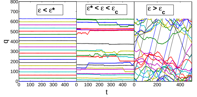
Fig. 1: A few tracer particles positions in the q -space as function of time. The analysis of the recorded trajectories clearly show that three dynamical regimes exist for the \beta -HMF model (3), depending on the energy per particle \varepsilon . At \varepsilon = \varepsilon^* , the perfect crystal like structure is lost, and the particles can wonder to neighboring sites. Above \varepsilon_c the self-organized crystal melts, resulting in a disordered gaseous medium. Here N = 500 , L = N and \alpha = 0.5 .
