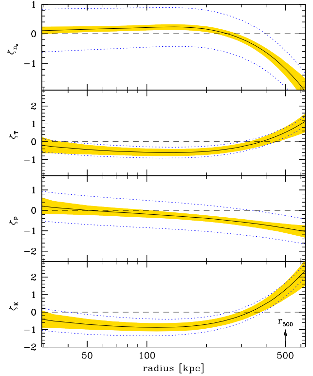
Figure 13. Evolutionary rates \zeta measured at fixed progenitor. Redshift evolution (slope with \log E(z) ) of the IDCS J1426.5+3508 thermodynamic profiles (mean value and 68 percent uncertainties, black line and yellow shading) when compared to its present-day expected descendants. The dotted corridor marks three times the X-COP scatter about the average. Negative values indicate deficits in the past, while the no-evolutionary case correspond to \zeta = 0 . The plot quantifies the evolutionary rates already appreciable in Fig. 12.
