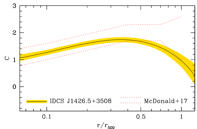
Figure 17. Electron density evolutionary rate C computed following McDonald et al. (2017). The evolution of the IDCS J1426.5+3508 electron density profile is indicated with the black line and yellow shading (mean value and 68 per cent uncertainties), and the McDonald et al. (2017) determination as the \pm 1\sigma dotted corridor. The low value of C at r \sim r_{500} indicates the need for a large gas density mass growth with this way of calculating the evolutionary rate.
