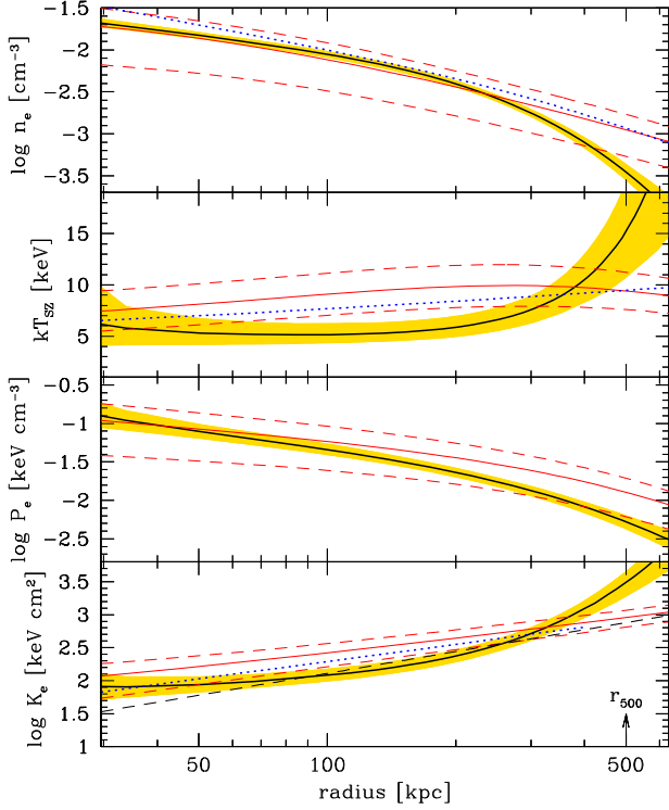
Figure 12. IDCS J1426.5+3508 (mean value and 68 percent uncertainties, black line, and yellow shading) is compared to its present-day expected descendant (red line with dashed corridor mark the mean value and the \pm 2\sigma , based on X-COP). Compared to its present-day descendant, at large radii gas is lacking and that present is too hot and with large entropy. To become a present-day cluster, heat and entropy should be dissipated or the gas transported to larger radii plus cold and low entropy gas should be acquired from peripheral regions. In electron density, temperature and entropy panels the profiles of Abell 2390, a possible IDCS J1426.5+3508 descendant, are shown with dotted blue line. Abell 2390 lacks a published pressure profile measurement.
