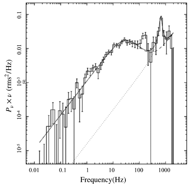
Figure 2. PDS in the normalized power ( P_v ) times frequency ( \nu ) representation, with the best-fitting multi-Lorentzian model.
