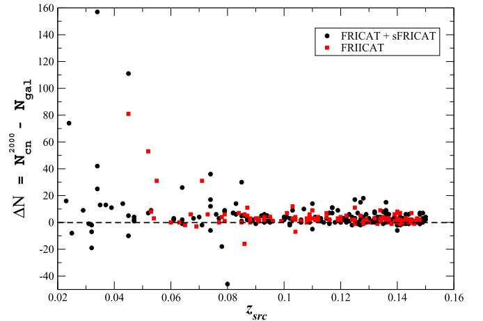
Figure 2. Difference, \Delta N , between the number of cosmological neighbors, N_{\text{cn}}^{2000} lying within 2 Mpc distance from the central RG and N_{\text{gal}} being the richness estimated in the T12 cluster catalog. Black circles mark radio sources in the FRICAT, including those of the sFRICAT, while red squares correspond to the FR IIs.
