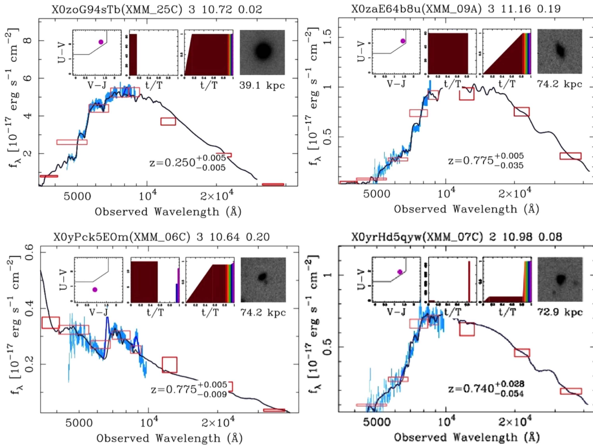
Figure 3. Examples of data and SEDs from the CSI survey. Each panel shows a plot of f_{\lambda} versus wavelength for photometric data (red boxes), spectroscopic data (cyan trace), and model SED (black line). The four small boxes above these contain derived data: (left) the UVJ diagram that separates star-forming from passive galaxies; (middle left) constant SFRs derived by the model for six time intervals, as described in the text; (middle right) integrated SFRs (stellar mass build-up) of the model; (right) the galaxy’s z -band image from the CFHT Legacy Survey.
